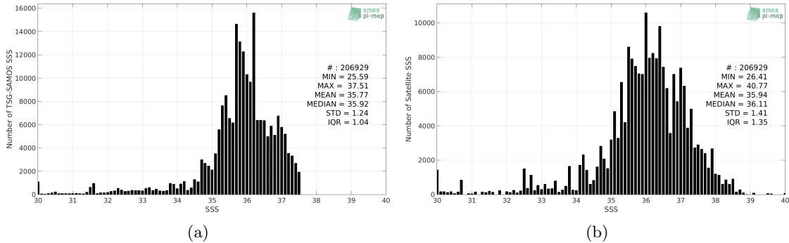
Figure 2: Histograms of SSS from TSG-SAMOS (a) and SMOS L2Q v321 - 0.25 Deg (CATDS-CPDC) (b) considering all match-up pairs per bins of 0.1 over the Tropical Atlantic Ocean Pi-MEP region and for the full satellite product period.
