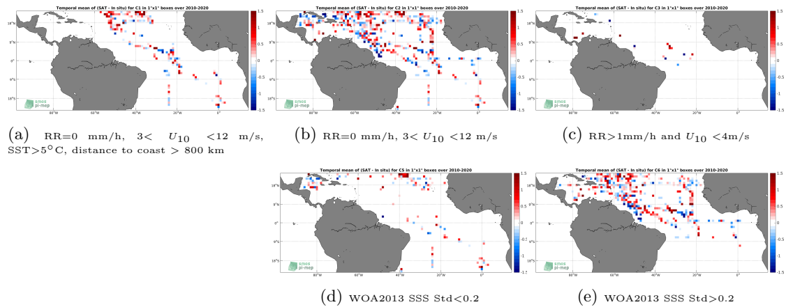
Figure 12: Temporal mean gridded over spatial boxes of size 1^\circ \times 1^\circ of \Delta SSS (SMOS L2Q v321 - 0.25 Deg (CATDS-CPDC) - TSG-SAMOS) for 5 different subdatasets corresponding to:RR=0 mm/h, 3 < U_{10} < 12 m/s, SST >5^\circ\text{C} , distance to coast > 800 km (a), RR=0 mm/h, 3 < U_{10} < 12 m/s (b), RR >1 mm/h and U_{10} < 4 m/s (c), WOA2013 SSS Std <0.2 (d), WOA2013 SSS Std >0.2 (e).
