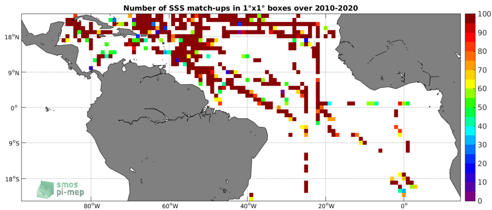
Figure 4: Number of SSS match-ups between TSG-SAMOS SSS and the SMOS L2Q v321 - 0.25 Deg (CATDS-CPDC) SSS product for the Tropical Atlantic Ocean Pi-MEP region over 1^\circ \times 1^\circ boxes and for the full satellite product period.
