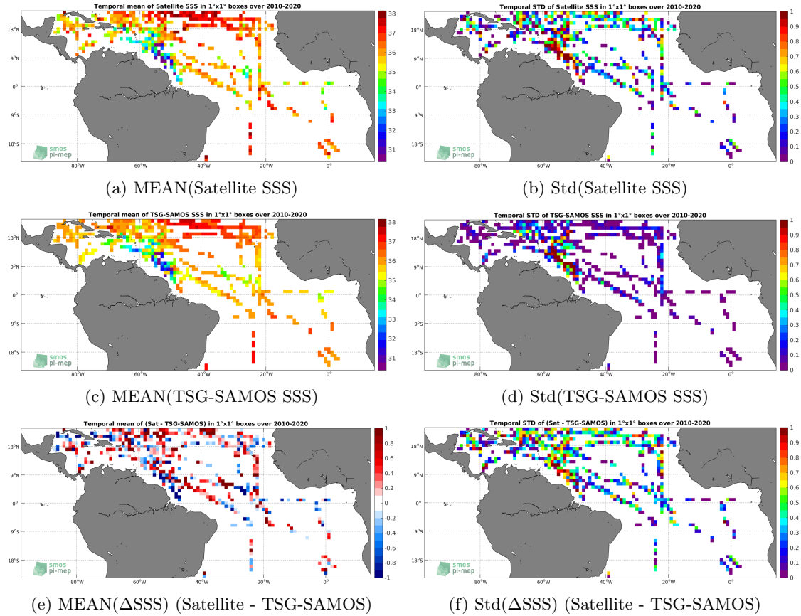
Figure 6: Temporal mean (left) and Std (right) of SSS from SMOS L2Q v321 - 0.25 Deg (CATDS-CPDC) (top), TSG-SAMOS (middle), and of \Delta SSS (Satellite - TSG-SAMOS). Only match-up pairs are used to generate these maps.
