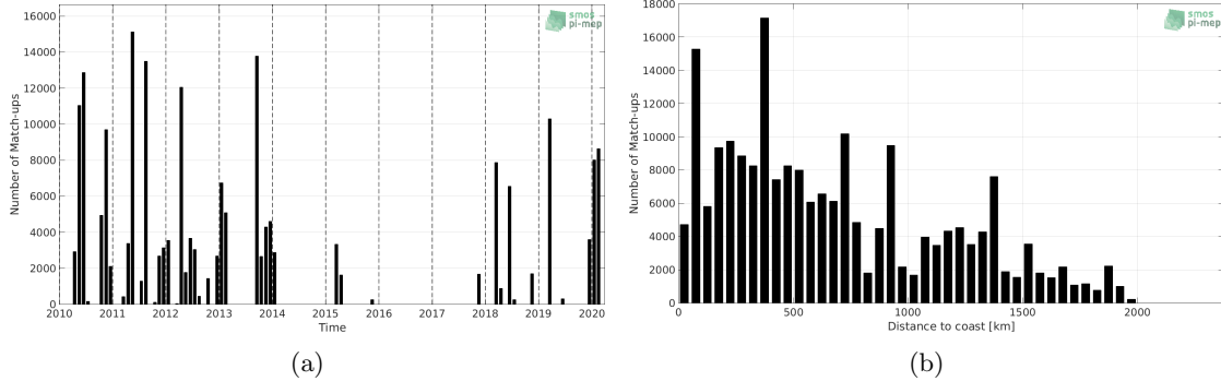
Figure 1: Number of match-ups between TSG-SAMOS and SMOS L2Q v321 - 0.25 Deg (CATDS-CPDC) SSS as a function of time (a) and as function of the distance to coast (b) over the Tropical Atlantic Ocean Pi-MEP region and for the full satellite product period.
