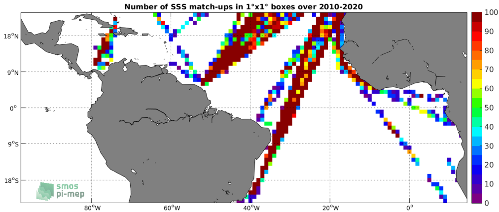
Figure 4: Number of SSS match-ups between TSG (LEGOS-DM) SSS and the SMOS SSS L2Q v321 - 0.25 Deg (CATDS-CPDC) SSS product for the Tropical Atlantic Ocean Pi-MEP region over 1^\circ \times 1^\circ boxes and for the full satellite product period.
