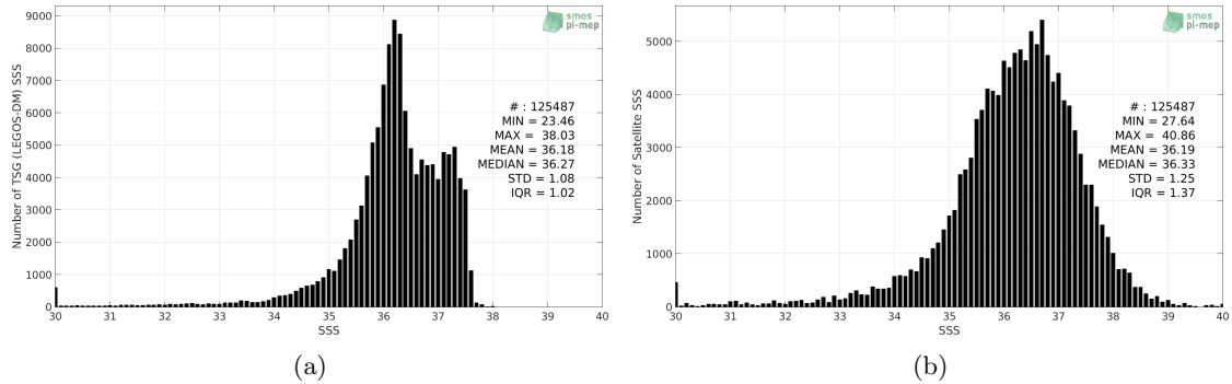
Figure 2: Histograms of SSS from TSG (LEGOS-DM) (a) and SMOS SSS L2Q v321 - 0.25 Deg (CATDS-CPDC) (b) considering all match-up pairs per bins of 0.1 over the Tropical Atlantic Ocean Pi-MEP region and for the full satellite product period.
