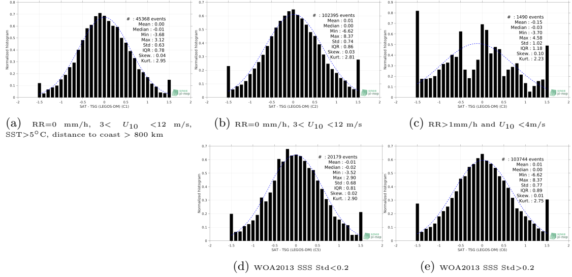
Figure 13: Normalized histogram of \Delta SSS (SMOS SSS L2Q v321 - 0.25 Deg (CATDS-CPDC) - TSG (LEGOS-DM)) for 5 different subdatasets corresponding to: RR=0 mm/h, 3 < U_{10} < 12 m/s, SST > 5°C, distance to coast > 800 km (a), RR=0 mm/h, 3 < U_{10} < 12 m/s (b), RR > 1mm/h and U_{10} < 4 m/s (c), WOA2013 SSS Std < 0.2 (d), WOA2013 SSS Std > 0.2 (e).
