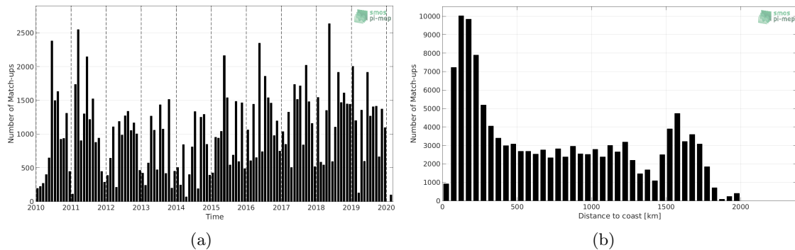
Figure 1: Number of match-ups between TSG (LEGOS-DM) and SMOS SSS L2Q v321 - 0.25 Deg (CATDS-CPDC) SSS as a function of time (a) and as function of the distance to coast (b) over the Tropical Atlantic Ocean Pi-MEP region and for the full satellite product period.
