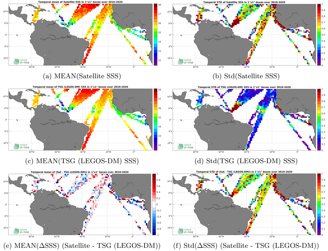
Figure 6: Temporal mean (left) and Std (right) of SSS from SMOS SSS L2Q v321 - 0.25 Deg (CATDS-CPDC) (top), TSG (LEGOS-DM) (middle), and of \Delta\text{SSS} (Satellite - TSG (LEGOS-DM)). Only match-up pairs are used to generate these maps.
