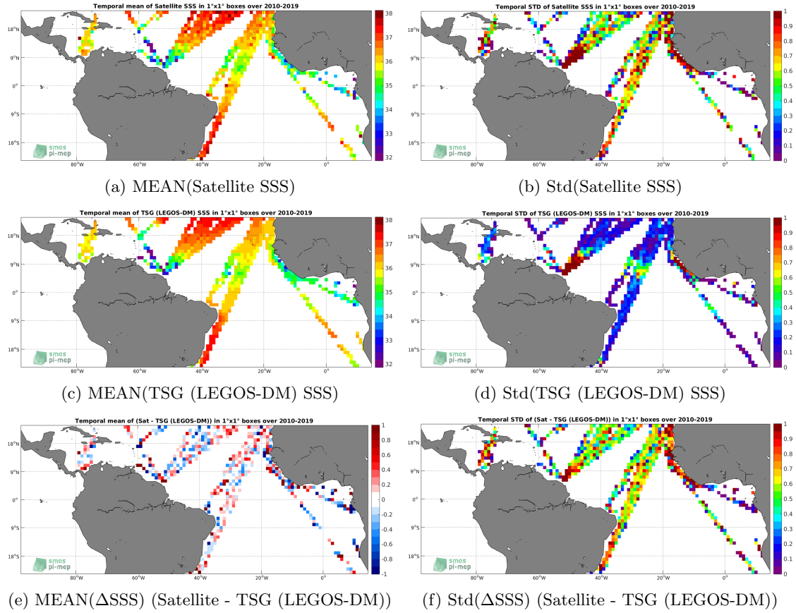
Figure 6: Temporal mean (left) and Std (right) of SSS from SMOS SSS L2Q v321 - 0.25 Deg (CATDS-CPDC) (top), TSG (LEGOS-DM) (middle), and of \Delta SSS (Satellite - TSG (LEGOS-DM)). Only match-up pairs are used to generate these maps.
