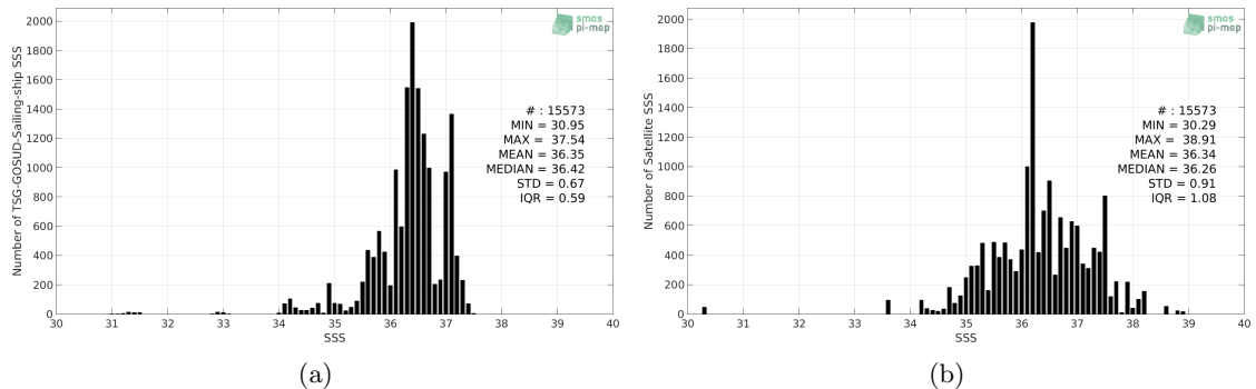
Figure 2: Histograms of SSS from TSG-GOSUD-Sailing-ship (a) and SMOS L2Q v321 - 0.25 Deg (CATDS-CPDC) (b) considering all match-up pairs per bins of 0.1 over the Tropical Atlantic Ocean Pi-MEP region and for the full satellite product period.
