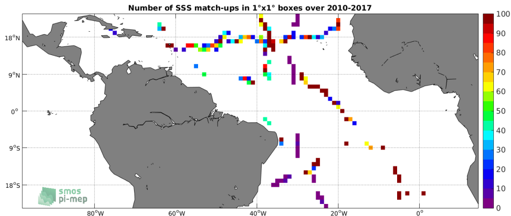
Figure 4: Number of SSS match-ups between TSG-GOSUD-Sailing-ship SSS and the SMOS L2Q v321 - 0.25 Deg (CATDS-CPDC) SSS product for the Tropical Atlantic Ocean Pi-MEP region over 1°x1° boxes and for the full satellite product period.
