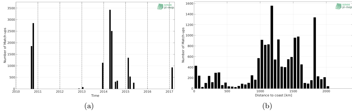
Figure 1: Number of match-ups between TSG-GOSUD-Sailing-ship and SMOS L2Q v321 - 0.25 Deg (CATDS-CPDC) SSS as a function of time (a) and as function of the distance to coast (b) over the Tropical Atlantic Ocean Pi-MEP region and for the full satellite product period.
