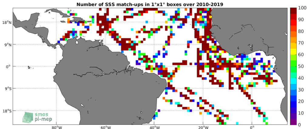
Figure 4: Number of SSS match-ups between TSG (GOSUD-Research-vessel) SSS and the SMOS SSS L2Q v321 - 0.25 Deg (CATDS-CPDC) SSS product for the Tropical Atlantic Ocean Pi-MEP region over 1°x1° boxes and for the full satellite product period.
