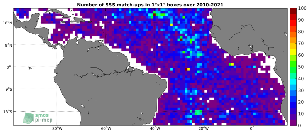
Figure 4: Number of SSS match-ups between Argo SSS and the SMOS SSS L2Q v321 - 0.25 Deg (CATDS-CPDC) SSS product for the Tropical Atlantic Ocean Pi-MEP region over 1°x1° boxes and for the full satellite product period.
