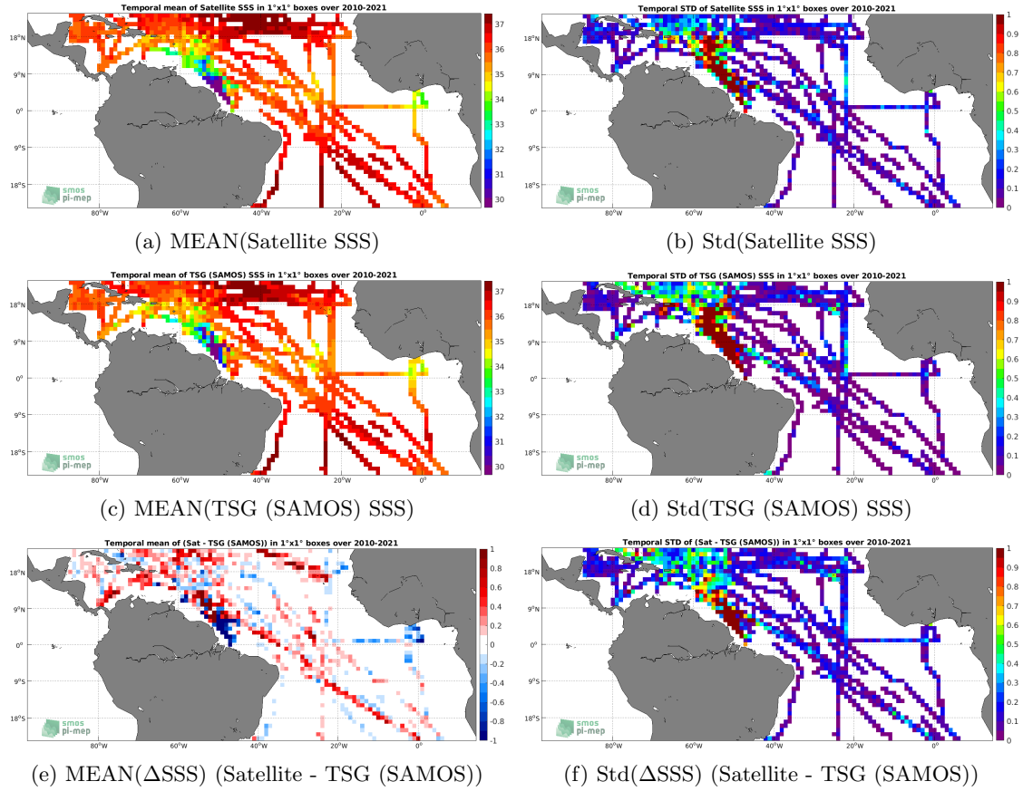
Figure 6: Temporal mean (left) and Std (right) of SSS from SMOS SSS L3 v317 - Monthly - 25 km (CATDS-CPDC) (top), TSG (SAMOS) (middle), and of \Delta SSS (Satellite - TSG (SAMOS)). Only match-up pairs are used to generate these maps.
