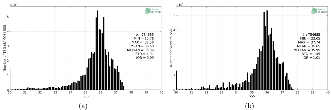
Figure 2: Histograms of SSS from TSG (SAMOS) (a) and SMOS SSS L3 v317 - Monthly - 25 km (CATDS-CPDC) (b) considering all match-up pairs per bins of 0.1 over the Tropical Atlantic Ocean Pi-MEP region and for the full satellite product period.
