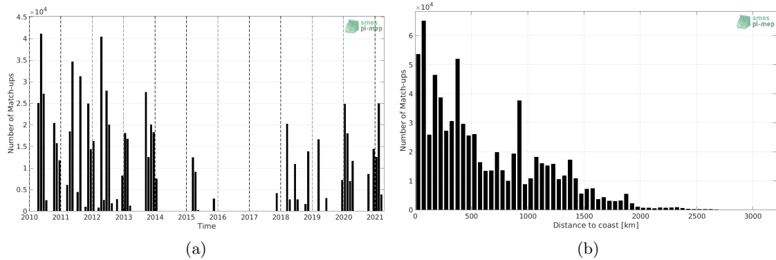
Figure 1: Number of match-ups between TSG (SAMOS) and SMOS SSS L3 v317 - Monthly - 25 km (CATDS-CPDC) SSS as a function of time (a) and as function of the distance to coast (b) over the Tropical Atlantic Ocean Pi-MEP region and for the full satellite product period.
