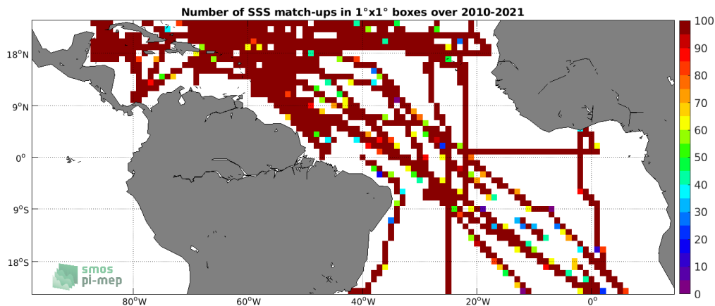
Figure 4: Number of SSS match-ups between TSG (SAMOS) SSS and the SMOS SSS L3 v317 - Monthly - 25 km (CATDS-CPDC) SSS product for the Tropical Atlantic Ocean Pi-MEP region over 1^\circ \times 1^\circ boxes and for the full satellite product period.
