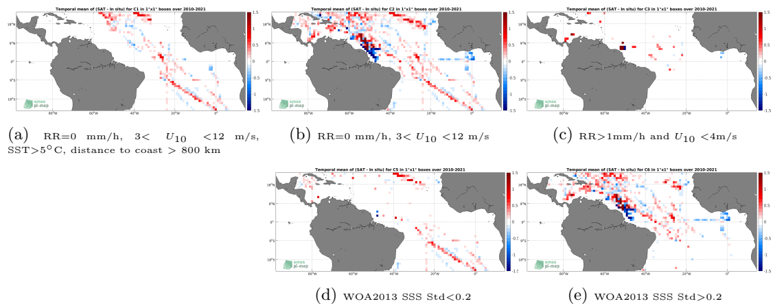
Figure 12: Temporal mean gridded over spatial boxes of size 1^\circ \times 1^\circ of \Delta SSS (SMOS SSS L3 v317 - Monthly - 25 km (CATDS-CPDC) - TSG (SAMOS)) for 5 different subdatasets corresponding to:RR=0 mm/h, 3 < U_{10} < 12 m/s, SST >5^\circ C, distance to coast > 800 km (a), RR=0 mm/h, 3 < U_{10} < 12 m/s (b), RR >1 mm/h and U_{10} < 4 m/s (c), WOA2013 SSS Std <0.2 (d), WOA2013 SSS Std >0.2 (e).
