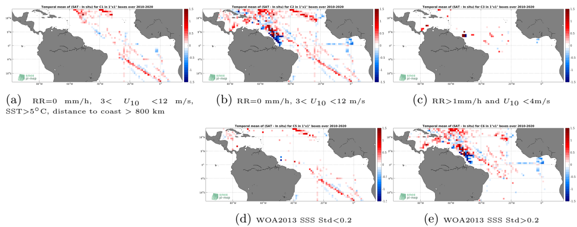
Figure 12: Temporal mean gridded over spatial boxes of size 1^\circ \times 1^\circ of \Delta\text{SSS} (SMOS SSS L3 v317 - Monthly - 25 km (CATDS-CPDC) - TSG (SAMOS)) for 5 different subdatasets corresponding to: RR=0 mm/h, 3 < U_{10} < 12 m/s, SST > 5°C, distance to coast > 800 km (a), RR=0 mm/h, 3 < U_{10} < 12 m/s (b), RR > 1mm/h and U_{10} < 4 m/s (c), WOA2013 SSS Std < 0.2 (d), WOA2013 SSS Std > 0.2 (e).
