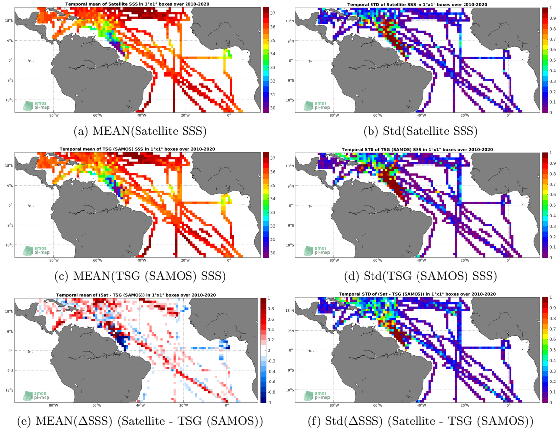
Figure 6: Temporal mean (left) and Std (right) of SSS from SMOS SSS L3 v317 - Monthly - 25 km (CATDS-CPDC) (top), TSG (SAMOS) ( in situ ) dataset (in blue) at the collected Pi-MEP match-up pairs. Only match-up pairs are used to generate these maps.
