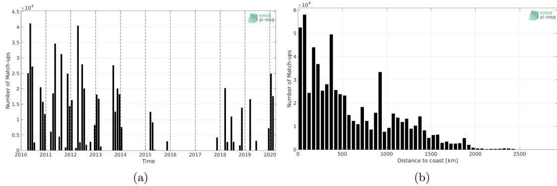
Figure 1: Number of match-ups between TSG-SAMOS and SMOS L3 v317 - Monthly - 25 km (CATDS-CPDC) SSS as a function of time (a) and as function of the distance to coast (b) over the Tropical Atlantic Ocean Pi-MEP region and for the full satellite product period.
