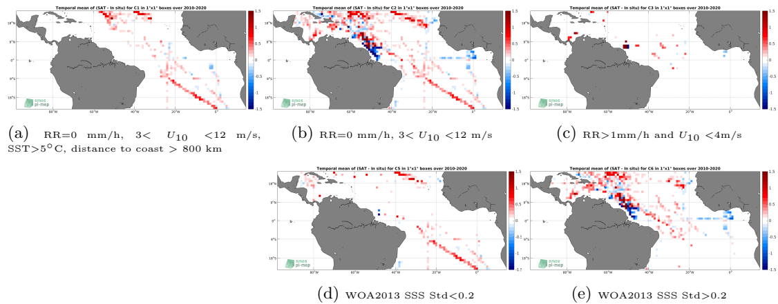
Figure 12: Temporal mean gridded over spatial boxes of size 1^\circ \times 1^\circ of \Delta SSS (SMOS L3 v317 - Monthly - 25 km (CATDS-CPDC) - TSG-SAMOS) for 5 different subdatasets corresponding to:RR=0 mm/h, 3 < U_{10} < 12 m/s, SST >5^\circ\text{C} , distance to coast > 800 km (a), RR=0 mm/h, 3 < U_{10} < 12 m/s (b), RR >1 mm/h and U_{10} < 4 m/s (c), WOA2013 SSS Std <0.2 (d), WOA2013 SSS Std >0.2 (e).
