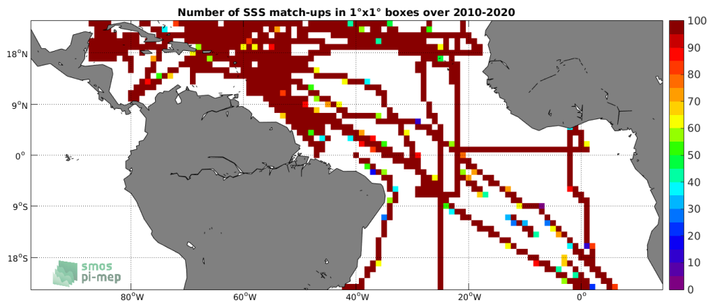
Figure 4: Number of SSS match-ups between TSG-SAMOS SSS and the SMOS L3 v317 - Monthly - 25 km (CATDS-CPDC) SSS product for the Tropical Atlantic Ocean Pi-MEP region over 1^\circ \times 1^\circ boxes and for the full satellite product period.
