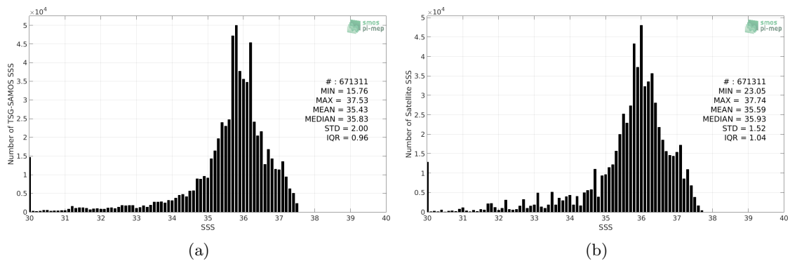
Figure 2: Histograms of SSS from TSG-SAMOS (a) and SMOS L3 v317 - Monthly - 25 km (CATDS-CPDC) (b) considering all match-up pairs per bins of 0.1 over the Tropical Atlantic Ocean Pi-MEP region and for the full satellite product period.
