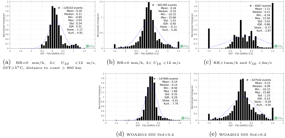
Figure 13: Normalized histogram of \Delta\text{SSS} (SMOS-L3-CATDS-CPDC-V317-MONTHLY-25KM - TSG-SAMOS) for 5 different subdatasets corresponding to: RR=0 mm/h, 3 < U_{10} < 12 m/s, SST>5°C, distance to coast > 800 km (a), RR=0 mm/h, 3 < U_{10} < 12 m/s (b), RR>1mm/h and U_{10} < 4 m/s (c), WOA2013 SSS Std<0.2 (d), WOA2013 SSS Std>0.2 (e).
