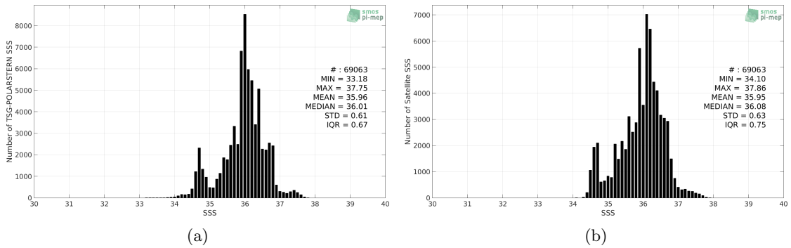
Figure 2: Histograms of SSS from TSG-POLARSTERN (a) and SMOS-L3-CATDS-CPDC-V317-MONTHLY-25KM (b) considering all match-up pairs per bins of 0.1 over the Tropical Atlantic Ocean Pi-MEP region and for the full satellite product period.
