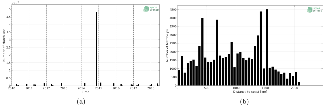
Figure 1: Number of match-ups between TSG-POLARSTERN and SMOS-L3-CATDS-CPDC-V317-MONTHLY-25KM SSS as a function of time (a) and as function of the distance to coast (b) over the Tropical Atlantic Ocean Pi-MEP region and for the full satellite product period.
