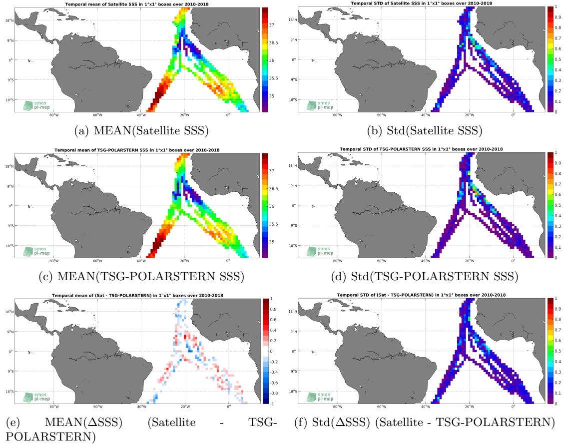
Figure 6: Temporal mean (left) and Std (right) of SSS from SMOS-L3-CATDS-CPDC-V317-MONTHLY-25KM (top), TSG-POLARSTERN (middle), and of \Delta SSS (Satellite - TSG-POLARSTERN). Only match-up pairs are used to generate these maps.
