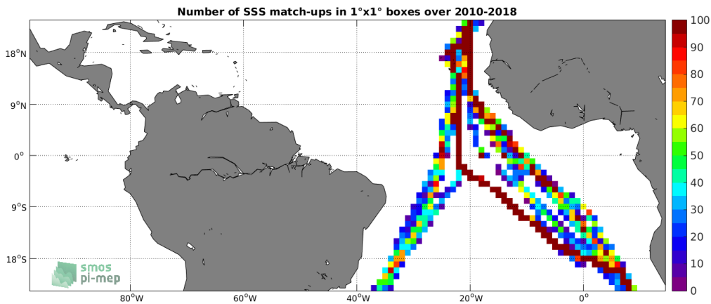
Figure 4: Number of SSS match-ups between TSG-POLARSTERN SSS and the SMOS-L3-CATDS-CPDC-V317-MONTHLY-25KM SSS product for the Tropical Atlantic Ocean Pi-MEP region over 1°x1° boxes and for the full satellite product period.
