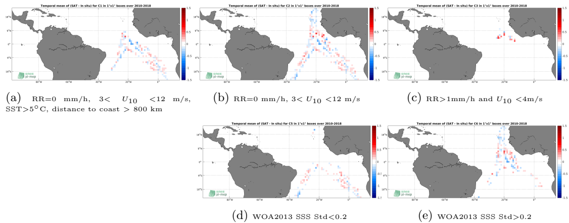
Figure 12: Temporal mean gridded over spatial boxes of size 1^\circ \times 1^\circ of \Delta SSS (SMOS-L3-CATDS-CPDC-V317-MONTHLY-25KM - TSG-POLARSTERN) for 5 different subdatasets corresponding to:RR=0 mm/h, 3 < U_{10} < 12 m/s, SST >5^\circ\text{C} , distance to coast > 800 km (a), RR=0 mm/h, 3 < U_{10} < 12 m/s (b), RR >1 mm/h and U_{10} < 4 m/s (c), WOA2013 SSS Std <0.2 (d), WOA2013 SSS Std >0.2 (e).
