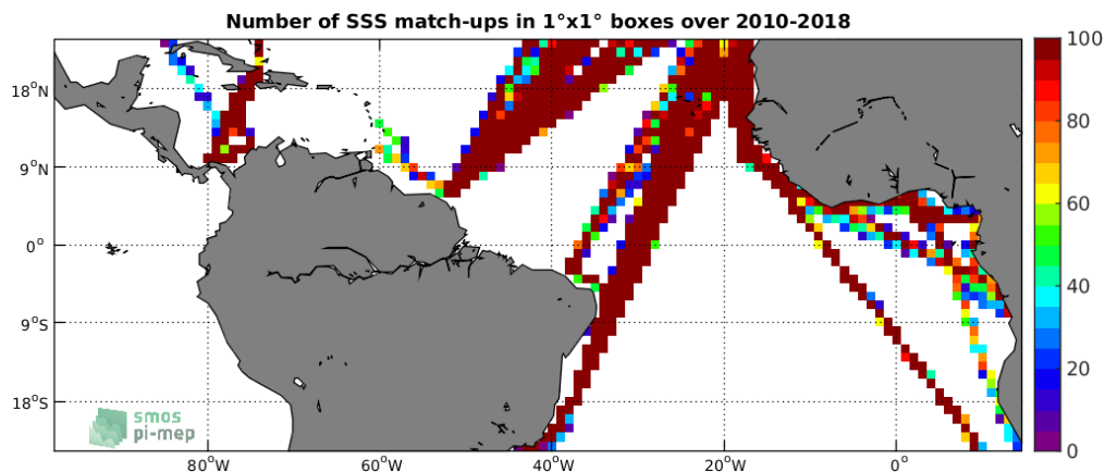
Figure 4: Number of SSS match-ups between TSG-LEGOS-DM SSS and the SMOS-L3-CATDS-CPDC-V317-MONTHLY-25KM SSS product for the Tropical Atlantic Ocean Pi-MEP region over 1^\circ \times 1^\circ boxes and for the full satellite product period.
