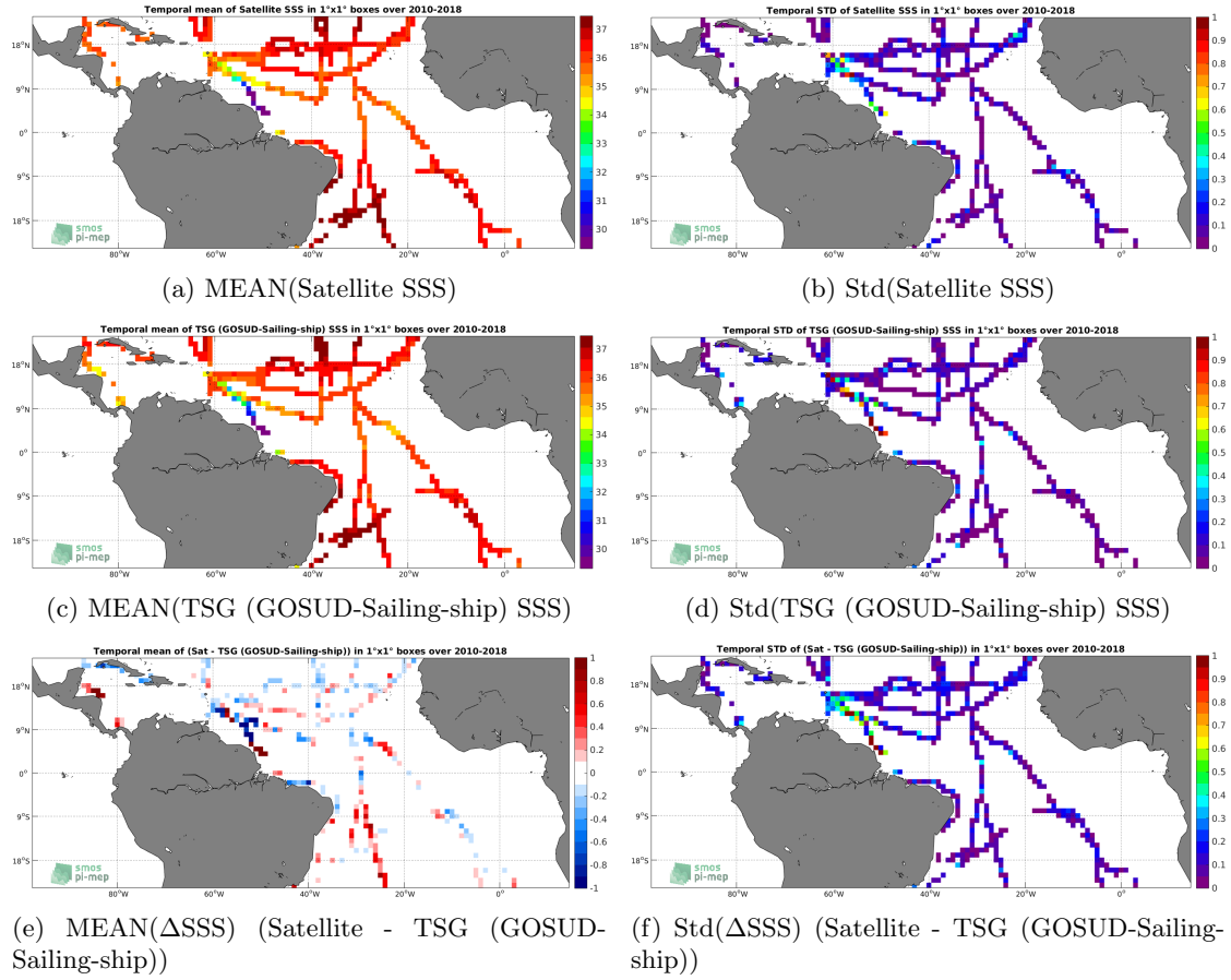
Figure 6: Temporal mean (left) and Std (right) of SSS from SMOS SSS L3 v317 - Monthly - 25 km (CATDS-CPDC) (top), TSG (GOSUD-Sailing-ship) (middle), and of \Delta SSS (Satellite - TSG (GOSUD-Sailing-ship)). Only match-up pairs are used to generate these maps.
