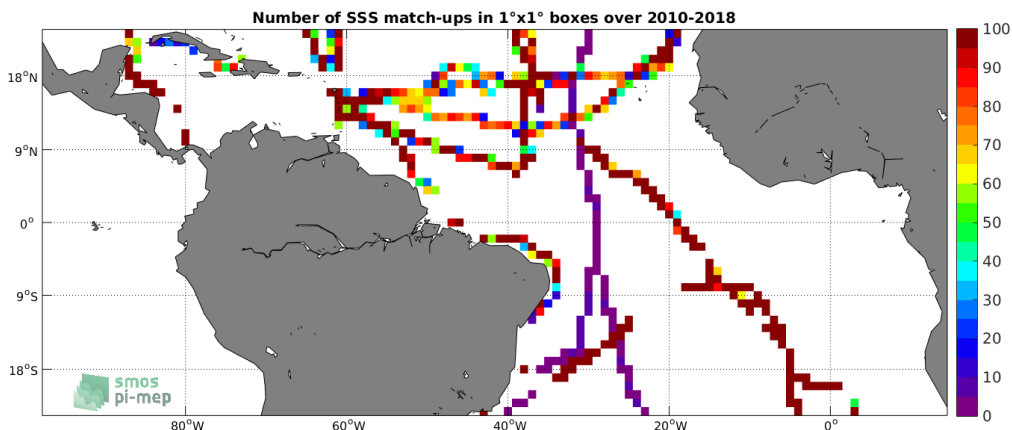
Figure 4: Number of SSS match-ups between TSG (GOSUD-Sailing-ship) SSS and the SMOS SSS L3 v317 - Monthly - 25 km (CATDS-CPDC) SSS product for the Tropical Atlantic Ocean Pi-MEP region over 1°x1° boxes and for the full satellite product period.
