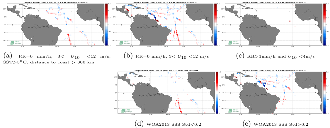
Figure 12: Temporal mean gridded over spatial boxes of size 1^\circ \times 1^\circ of \Delta SSS (SMOS SSS L3 v317 - Monthly - 25 km (CATDS-CPDC) - TSG (GOSUD-Sailing-ship)) for 5 different subdatasets corresponding to:RR=0 mm/h, 3 < U_{10} < 12 m/s, SST >5^\circ\text{C} , distance to coast > 800 km (a), RR=0 mm/h, 3 < U_{10} < 12 m/s (b), RR >1 mm/h and U_{10} < 4 m/s (c), WOA2013 SSS Std <0.2 (d), WOA2013 SSS Std >0.2 (e).
