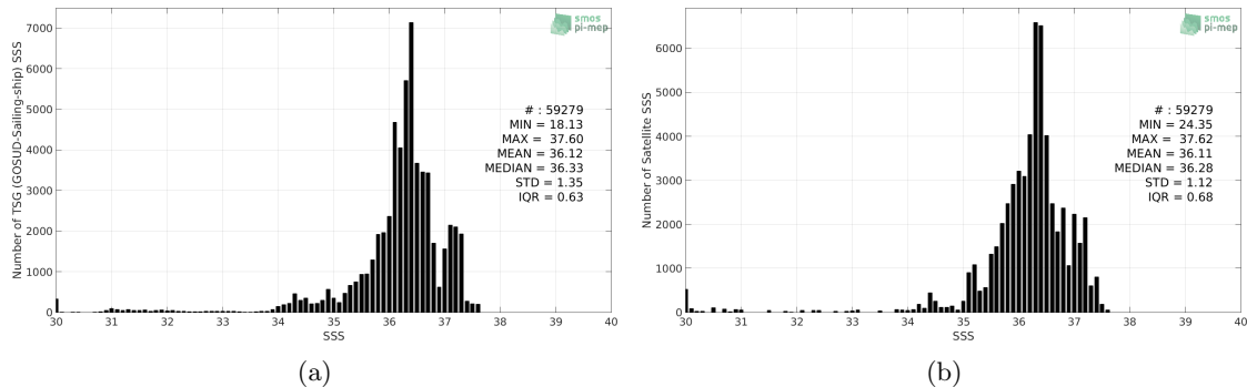
Figure 2: Histograms of SSS from TSG (GOSUD-Sailing-ship) (a) and SMOS SSS L3 v317 - Monthly - 25 km (CATDS-CPDC) (b) considering all match-up pairs per bins of 0.1 over the Tropical Atlantic Ocean Pi-MEP region and for the full satellite product period.
