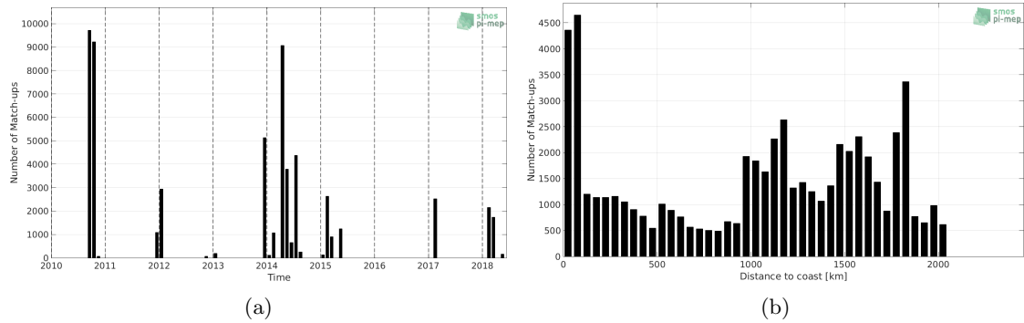
Figure 1: Number of match-ups between TSG (GOSUD-Sailing-ship) and SMOS SSS L3 v317 - Monthly - 25 km (CATDS-CPDC) SSS as a function of time (a) and as function of the distance to coast (b) over the Tropical Atlantic Ocean Pi-MEP region and for the full satellite product period.
