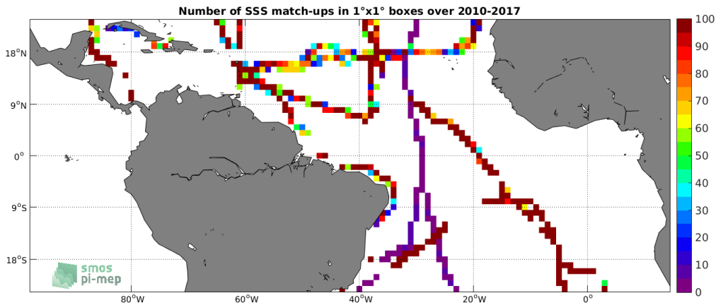
Figure 4: Number of SSS match-ups between TSG (GOSUD-Sailing-ship) SSS and the SMOS SSS L3 v317 - Monthly - 25 km (CATDS-CPDC) SSS product for the Tropical Atlantic Ocean Pi-MEP region over 1^\circ \times 1^\circ boxes and for the full satellite product period.
