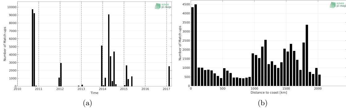
Figure 1: Number of match-ups between TSG-GOSUD-Sailing-ship and SMOS L3 v317 - Monthly - 25 km (CATDS-CPDC) SSS as a function of time (a) and as function of the distance to coast (b) over the Tropical Atlantic Ocean Pi-MEP region and for the full satellite product period.
