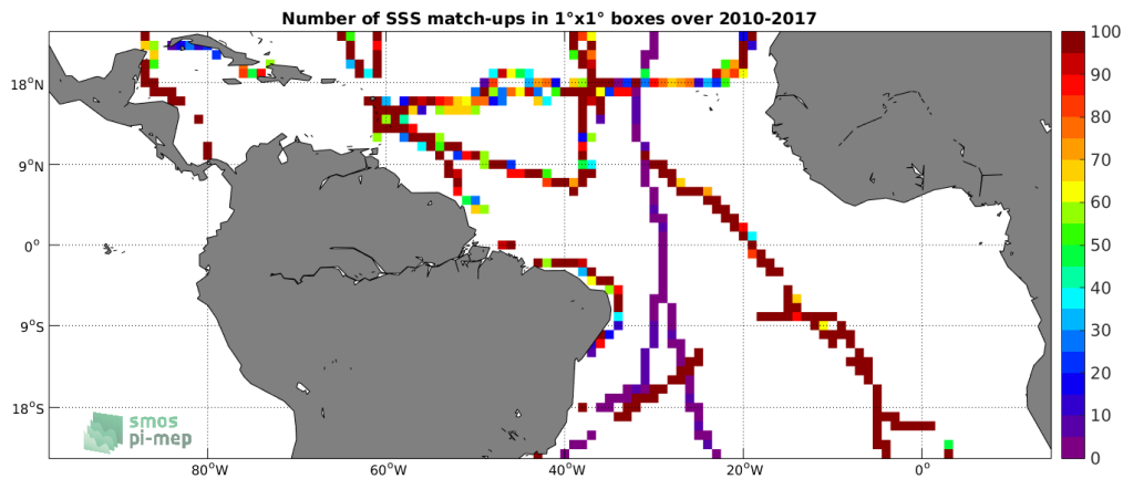
Figure 4: Number of SSS match-ups between TSG-GOSUD-Sailing-ship SSS and the SMOS L3 v317 - Monthly - 25 km (CATDS-CPDC) SSS product for the Tropical Atlantic Ocean Pi-MEP region over 1^\circ \times 1^\circ boxes and for the full satellite product period.
