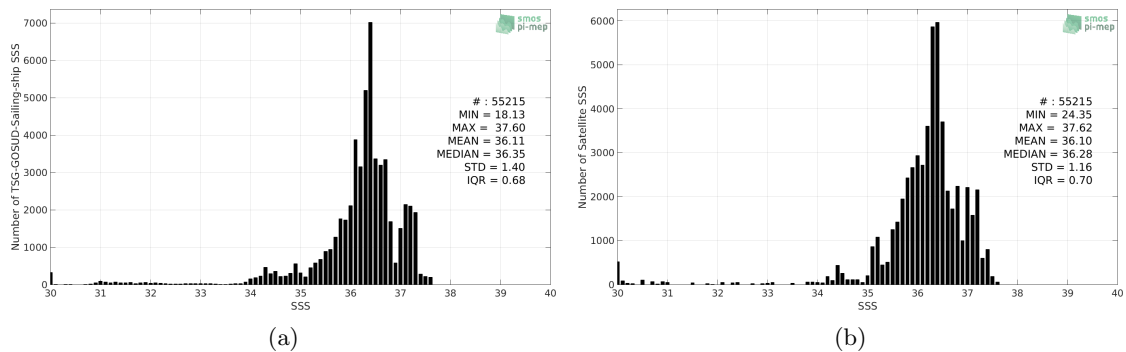
Figure 2: Histograms of SSS from TSG-GOSUD-Sailing-ship (a) and SMOS L3 v317 - Monthly - 25 km (CATDS-CPDC) (b) considering all match-up pairs per bins of 0.1 over the Tropical Atlantic Ocean Pi-MEP region and for the full satellite product period.
