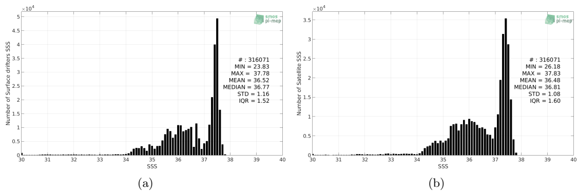
Figure 2: Histograms of SSS from Surface drifters (a) and SMOS L3 v317 - Monthly - 25 km (CATDS-CPDC) (b) considering all match-up pairs per bins of 0.1 over the Tropical Atlantic Ocean Pi-MEP region and for the full satellite product period.
