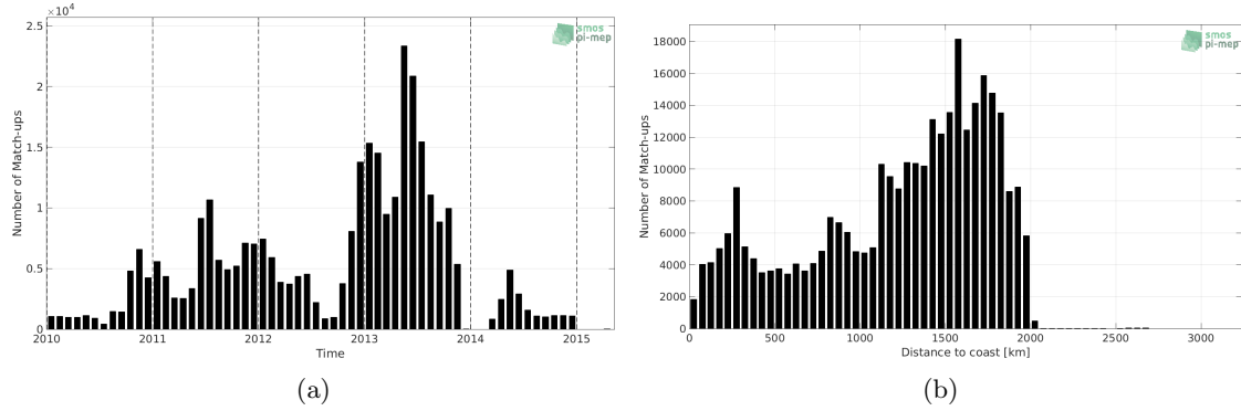
Figure 1: Number of match-ups between Surface drifters and SMOS L3 v317 - Monthly - 25 km (CATDS-CPDC) SSS as a function of time (a) and as function of the distance to coast (b) over the Tropical Atlantic Ocean Pi-MEP region and for the full satellite product period.
