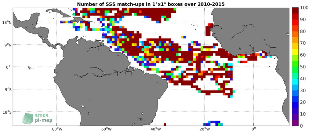
Figure 3: Number of SSS match-ups between Surface drifters SSS and the SMOS L3 v317 - Monthly - 25 km (CATDS-CPDC) SSS product for the Tropical Atlantic Ocean Pi-MEP region over 1^\circ \times 1^\circ boxes and for the full satellite product period.
