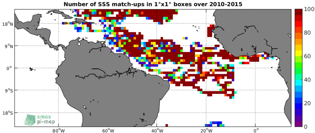
Figure 3: Number of SSS match-ups between Surface drifters SSS and the SMOS-L3-CATDS-CPDC-V317-MONTHLY-25KM SSS product for the Tropical Atlantic Ocean Pi-MEP region over 1^\circ \times 1^\circ boxes and for the full satellite product period.
