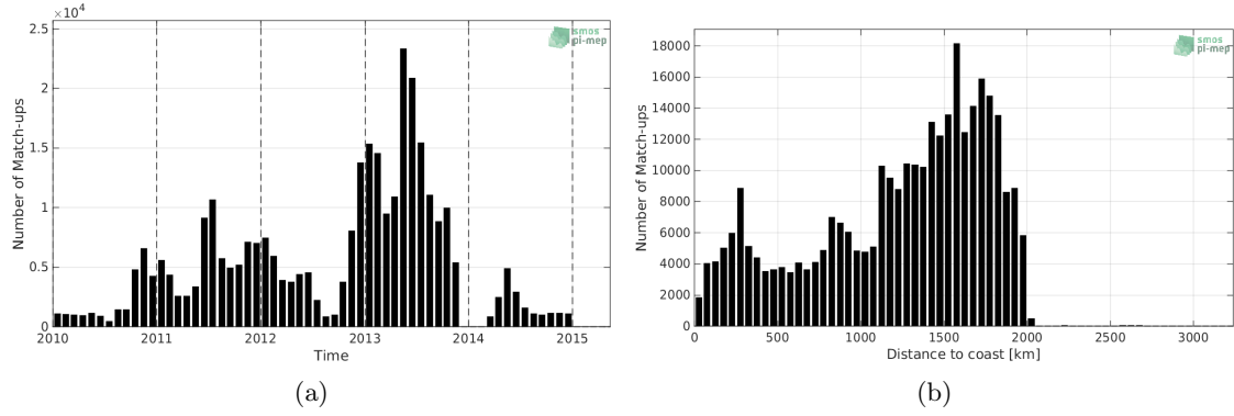
Figure 1: Number of match-ups between Surface drifters and SMOS-L3-CATDS-CPDC-V317-MONTHLY-25KM SSS as a function of time (a) and as function of the distance to coast (b) over the Tropical Atlantic Ocean Pi-MEP region and for the full satellite product period.
