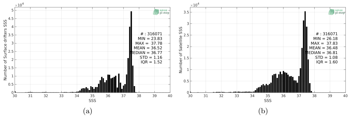
Figure 2: Histograms of SSS from Surface drifters (a) and SMOS-L3-CATDS-CPDC-V317-MONTHLY-25KM (b) considering all match-up pairs per bins of 0.1 over the Tropical Atlantic Ocean Pi-MEP region and for the full satellite product period.
