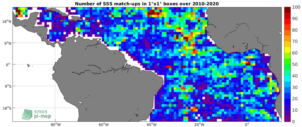
Figure 4: Number of SSS match-ups between Argo SSS and the SMOS SSS L3 v317 - Monthly - 25 km (CATDS-CPDC) SSS product for the Tropical Atlantic Ocean Pi-MEP region over 1^\circ \times 1^\circ boxes and for the full satellite product period.
