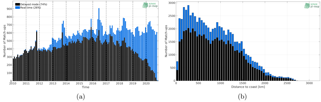
Figure 1: Number of match-ups between Argo and SMOS SSS L3 v317 - Monthly - 25 km (CATDS-CPDC) SSS as a function of time (a) and as function of the distance to coast (b) over the Tropical Atlantic Ocean Pi-MEP region and for the full satellite product period.
