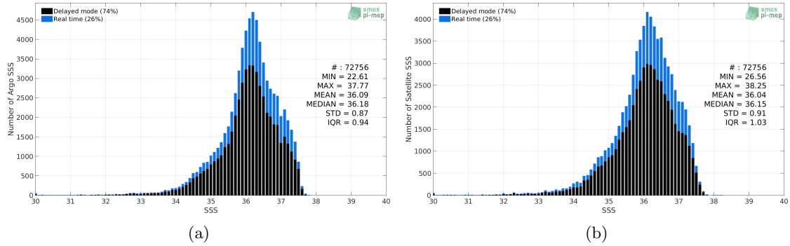
Figure 2: Histograms of SSS from Argo (a) and SMOS SSS L3 v317 - Monthly - 25 km (CATDS-CPDC) (b) considering all match-up pairs per bins of 0.1 over the Tropical Atlantic Ocean Pi-MEP region and for the full satellite product period.
