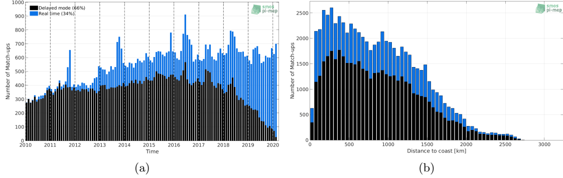
Figure 1: Number of match-ups between Argo and SMOS L3 v317 - Monthly - 25 km (CATDS-CPDC) SSS as a function of time (a) and as function of the distance to coast (b) over the Tropical Atlantic Ocean Pi-MEP region and for the full satellite product period.
