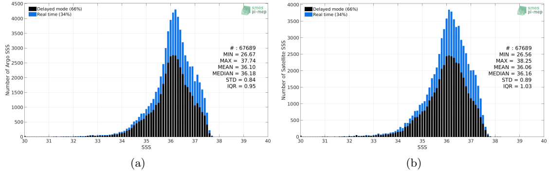
Figure 2: Histograms of SSS from Argo (a) and SMOS L3 v317 - Monthly - 25 km (CATDS-CPDC) (b) considering all match-up pairs per bins of 0.1 over the Tropical Atlantic Ocean Pi-MEP region and for the full satellite product period.
