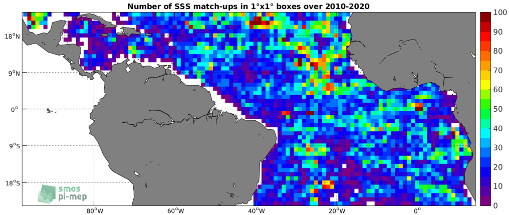
Figure 4: Number of SSS match-ups between Argo SSS and the SMOS L3 v317 - Monthly - 25 km (CATDS-CPDC) SSS product for the Tropical Atlantic Ocean Pi-MEP region over 1°x1° boxes and for the full satellite product period.
