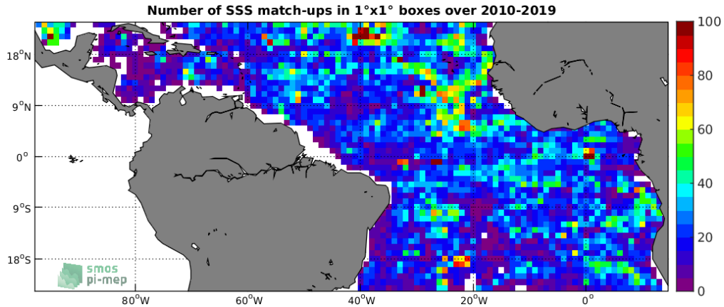
Figure 4: Number of SSS match-ups between Argo SSS and the SMOS-L3-CATDS-CPDC-V317-MONTHLY-25KM SSS product for the Tropical Atlantic Ocean Pi-MEP region over 1^\circ \times 1^\circ boxes and for the full satellite product period.
