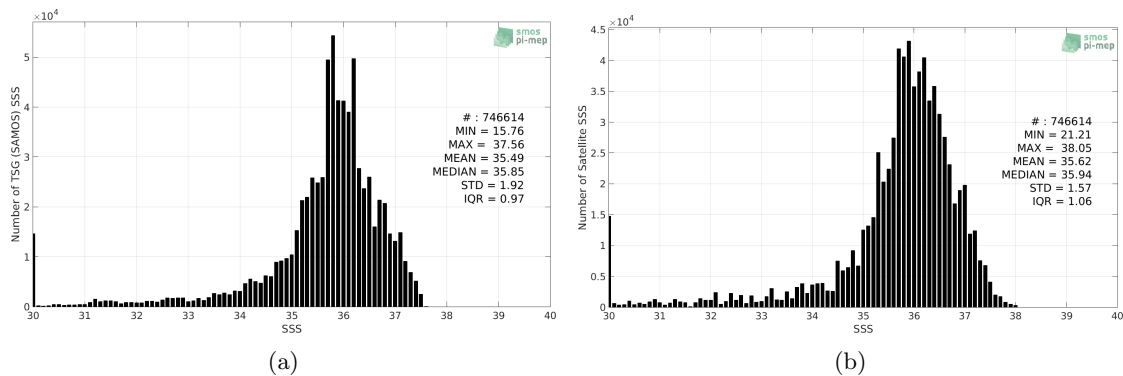
Figure 2: Histograms of SSS from TSG (SAMOS) (a) and SMOS SSS L3 v317 - 10 Days - 25 km (CATDS-CPDC) (b) considering all match-up pairs per bins of 0.1 over the Tropical Atlantic Ocean Pi-MEP region and for the full satellite product period.
