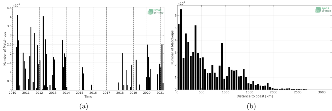
Figure 1: Number of match-ups between TSG (SAMOS) and SMOS SSS L3 v317 - 10 Days - 25 km (CATDS-CPDC) SSS as a function of time (a) and as function of the distance to the coast (b) over the Tropical Atlantic Ocean Pi-MEP region and for the full satellite product period.
