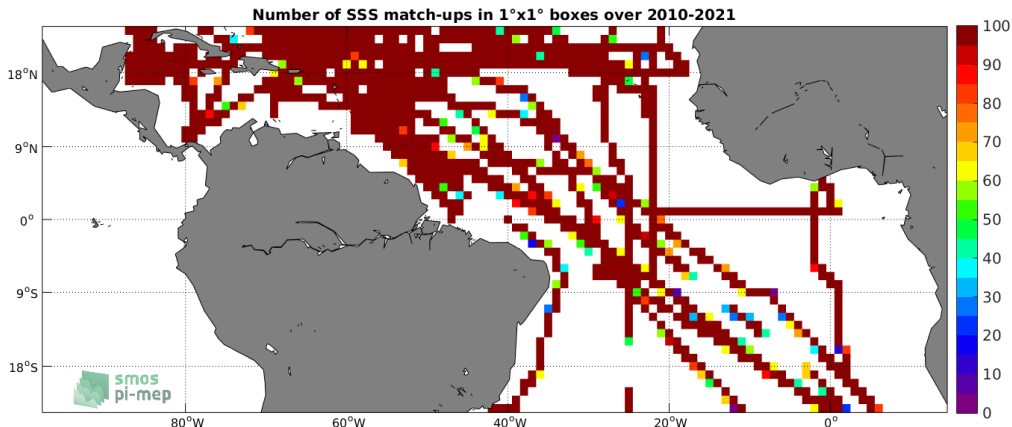
Figure 4: Number of SSS match-ups between TSG (SAMOS) SSS and the SMOS SSS L3 v317 - 10 Days - 25 km (CATDS-CPDC) SSS product for the Tropical Atlantic Ocean Pi-MEP region over 1^\circ \times 1^\circ boxes and for the full satellite product period.
