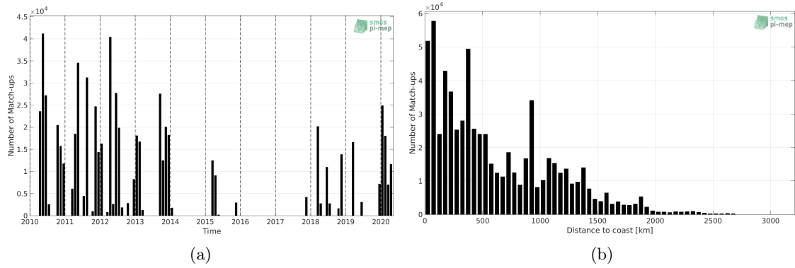
Figure 1: Number of match-ups between TSG (SAMOS) and SMOS SSS L3 v317 - 10 Days - 25 km (CATDS-CPDC) SSS as a function of time (a) and as function of the distance to coast (b) over the Tropical Atlantic Ocean Pi-MEP region and for the full satellite product period.
