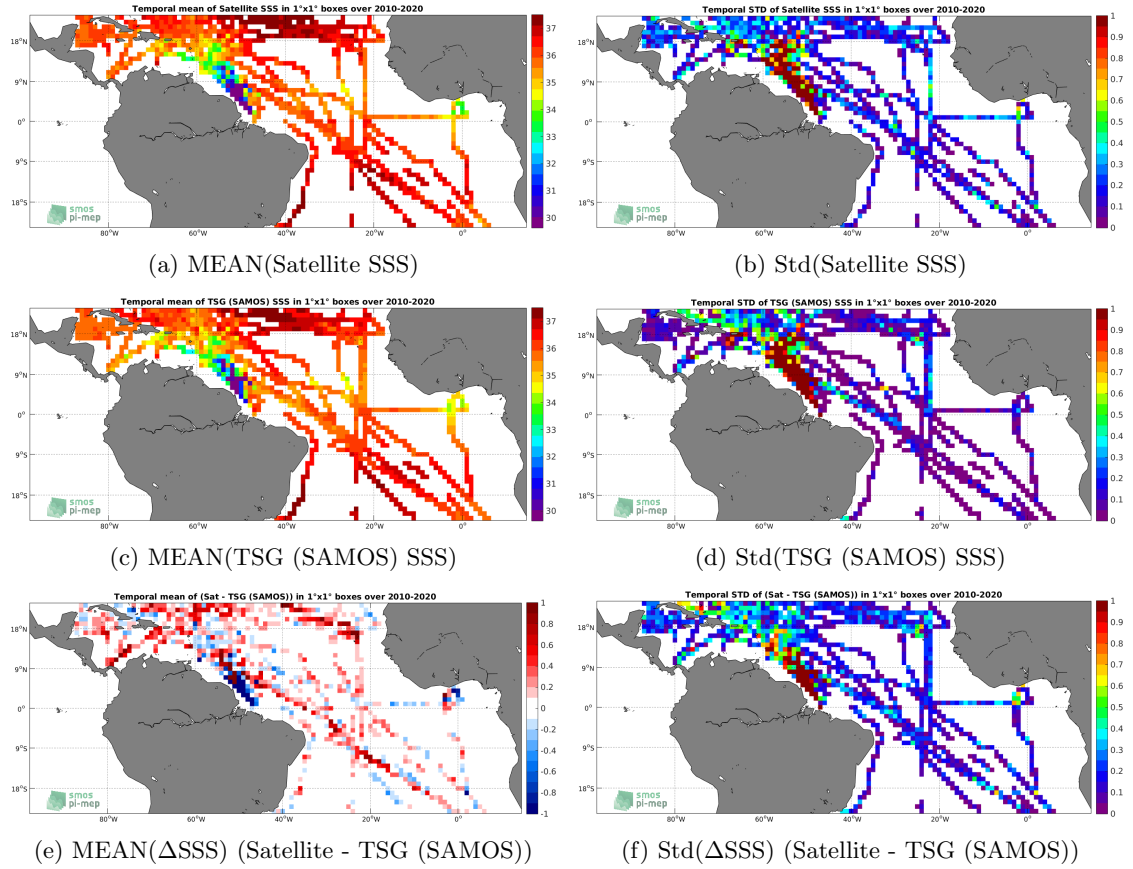
Figure 6: Temporal mean (left) and Std (right) of SSS from SMOS SSS L3 v317 - 10 Days - 25 km (CATDS-CPDC) (top), TSG (SAMOS) ( in situ ) dataset (middle), and of \Delta SSS (Satellite - TSG (SAMOS)). Only match-up pairs are used to generate these maps.
