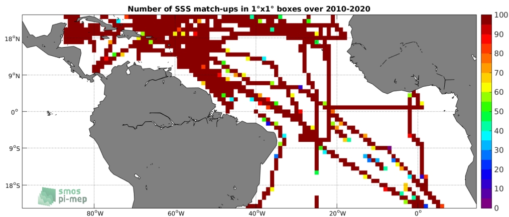
Figure 4: Number of SSS match-ups between TSG-SAMOS SSS and the SMOS L3 v317 - 10 Days - 25 km (CATDS-CPDC) SSS product for the Tropical Atlantic Ocean Pi-MEP region over 1^\circ \times 1^\circ boxes and for the full satellite product period.
