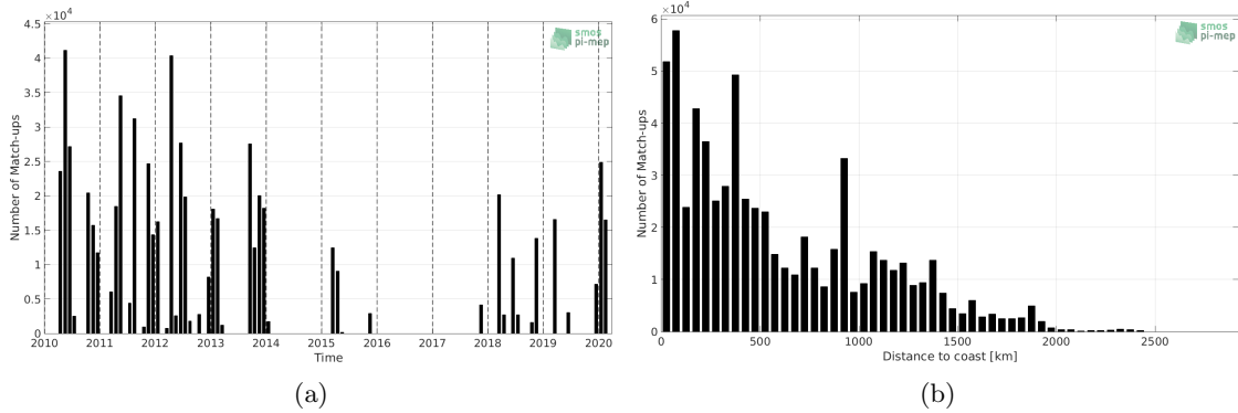
Figure 1: Number of match-ups between TSG-SAMOS and SMOS L3 v317 - 10 Days - 25 km (CATDS-CPDC) SSS as a function of time (a) and as function of the distance to coast (b) over the Tropical Atlantic Ocean Pi-MEP region and for the full satellite product period.
