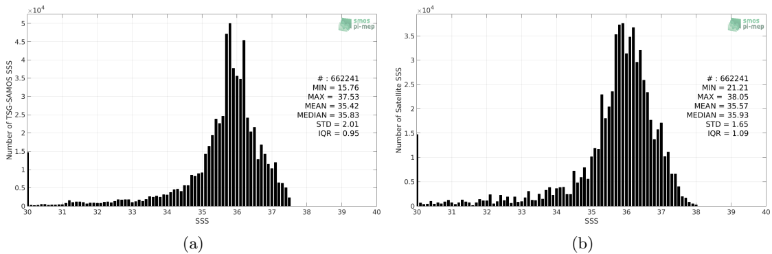
Figure 2: Histograms of SSS from TSG-SAMOS (a) and SMOS L3 v317 - 10 Days - 25 km (CATDS-CPDC) (b) considering all match-up pairs per bins of 0.1 over the Tropical Atlantic Ocean Pi-MEP region and for the full satellite product period.
