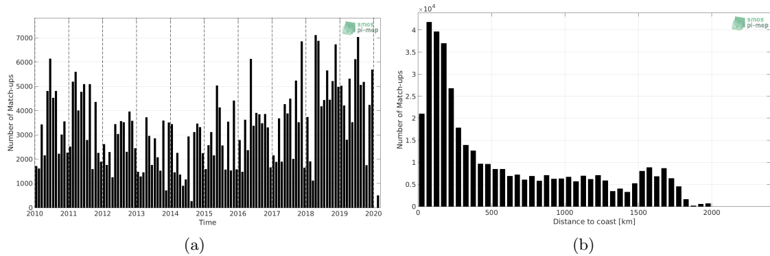
Figure 1: Number of match-ups between TSG (LEGOS-DM) and SMOS SSS L3 v317 - 10 Days - 25 km (CATDS-CPDC) SSS as a function of time (a) and as function of the distance to coast (b) over the Tropical Atlantic Ocean Pi-MEP region and for the full satellite product period.
