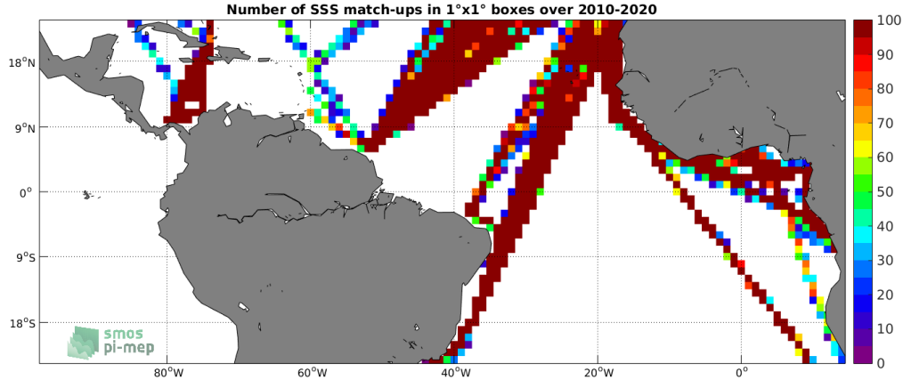
Figure 4: Number of SSS match-ups between TSG (LEGOS-DM) SSS and the SMOS SSS L3 v317 - 10 Days - 25 km (CATDS-CPDC) SSS product for the Tropical Atlantic Ocean Pi-MEP region over 1^\circ \times 1^\circ boxes and for the full satellite product period.
