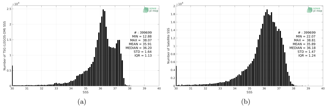
Figure 2: Histograms of SSS from TSG (LEGOS-DM) (a) and SMOS SSS L3 v317 - 10 Days - 25 km (CATDS-CPDC) (b) considering all match-up pairs per bins of 0.1 over the Tropical Atlantic Ocean Pi-MEP region and for the full satellite product period.
