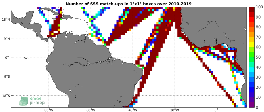
Figure 4: Number of SSS match-ups between TSG-LEGOS-DM SSS and the SMOS L3 v317 - 10 Days - 25 km (CATDS-CPDC) SSS product for the Tropical Atlantic Ocean Pi-MEP region over 1^\circ \times 1^\circ boxes and for the full satellite product period.
