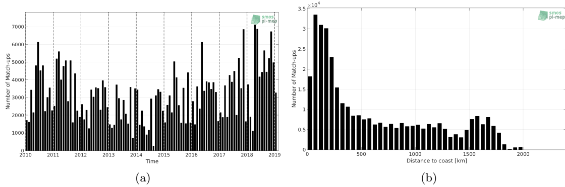
Figure 1: Number of match-ups between TSG-LEGOS-DM and SMOS L3 v317 - 10 Days - 25 km (CATDS-CPDC) SSS as a function of time (a) and as function of the distance to coast (b) over the Tropical Atlantic Ocean Pi-MEP region and for the full satellite product period.
