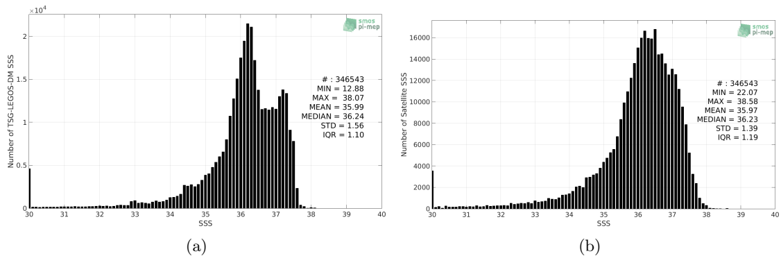
Figure 2: Histograms of SSS from TSG-LEGOS-DM (a) and SMOS L3 v317 - 10 Days - 25 km (CATDS-CPDC) (b) considering all match-up pairs per bins of 0.1 over the Tropical Atlantic Ocean Pi-MEP region and for the full satellite product period.
