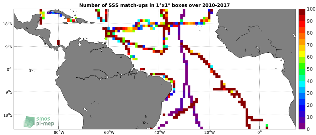
Figure 4: Number of SSS match-ups between TSG-GOSUD-Sailing-ship SSS and the SMOS L3 v317 - 10 Days - 25 km (CATDS-CPDC) SSS product for the Tropical Atlantic Ocean Pi-MEP region over 1^\circ \times 1^\circ boxes and for the full satellite product period.
