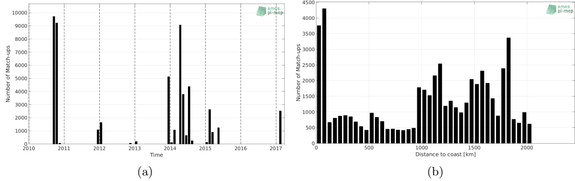
Figure 1: Number of match-ups between TSG-GOSUD-Sailing-ship and SMOS L3 v317 - 10 Days - 25 km (CATDS-CPDC) SSS as a function of time (a) and as function of the distance to coast (b) over the Tropical Atlantic Ocean Pi-MEP region and for the full satellite product period.
