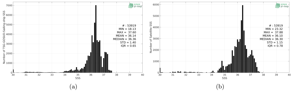
Figure 2: Histograms of SSS from TSG-GOSUD-Sailing-ship (a) and SMOS L3 v317 - 10 Days - 25 km (CATDS-CPDC) (b) considering all match-up pairs per bins of 0.1 over the Tropical Atlantic Ocean Pi-MEP region and for the full satellite product period.
