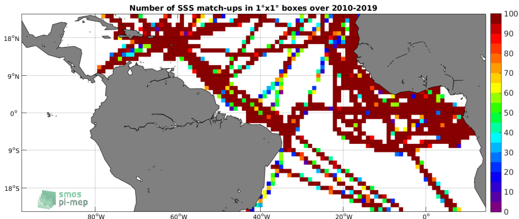
Figure 4: Number of SSS match-ups between TSG (GOSUD-Research-vessel) SSS and the SMOS SSS L3 v317 - 10 Days - 25 km (CATDS-CPDC) SSS product for the Tropical Atlantic Ocean Pi-MEP region over 1°x1° boxes and for the full satellite product period.
