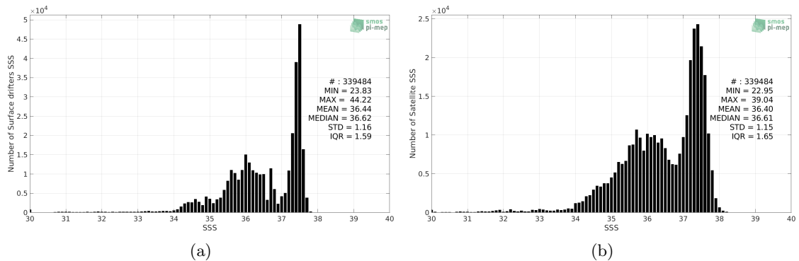
Figure 2: Histograms of SSS from Surface drifters (a) and SMOS SSS L3 v317 - 10 Days - 25 km (CATDS-CPDC) (b) considering all match-up pairs per bins of 0.1 over the Tropical Atlantic Ocean Pi-MEP region and for the full satellite product period.
