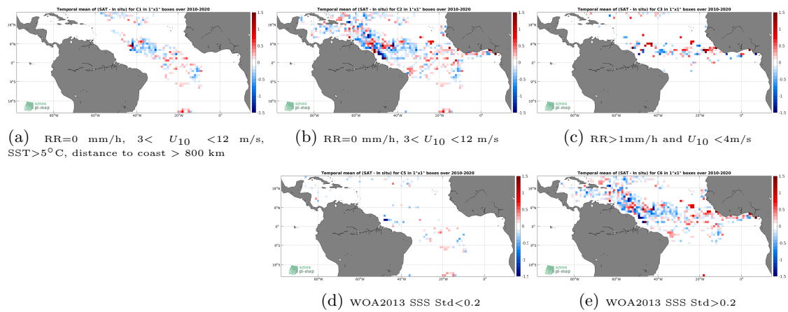
Figure 11: Temporal mean gridded over spatial boxes of size 1^\circ \times 1^\circ of \Delta\text{SSS} (SMOS SSS L3 v317 - 10 Days - 25 km (CATDS-CPDC) - Surface drifters) for 5 different subdatasets corresponding to:RR=0 mm/h, 3 < U_{10} < 12 m/s, SST >5^\circ\text{C} , distance to coast > 800 km (a), RR=0 mm/h, 3 < U_{10} < 12 m/s (b), RR >1 mm/h and U_{10} < 4 m/s (c), WOA2013 SSS Std <0.2 (d), WOA2013 SSS Std >0.2 (e).
