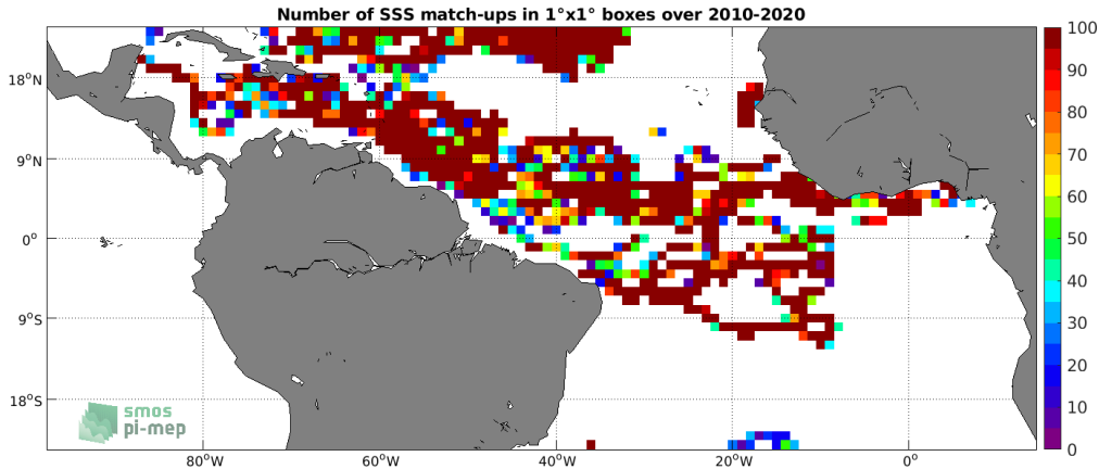
Figure 3: Number of SSS match-ups between Surface drifters SSS and the SMOS SSS L3 v317 - 10 Days - 25 km (CATDS-CPDC) SSS product for the Tropical Atlantic Ocean Pi-MEP region over 1^\circ \times 1^\circ boxes and for the full satellite product period.
