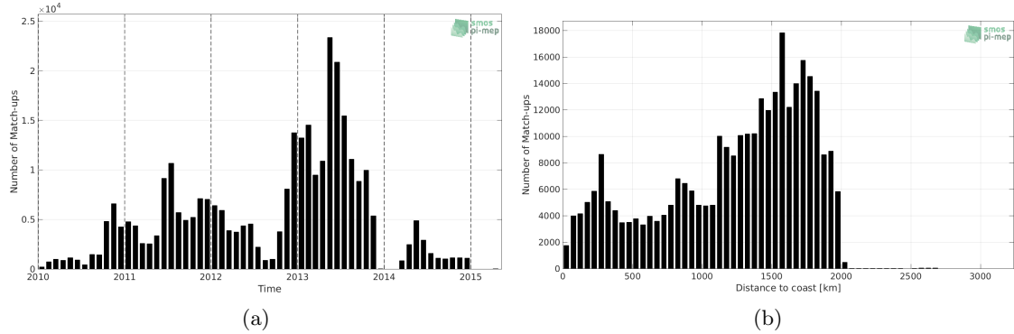
Figure 1: Number of match-ups between Surface drifters and SMOS SSS L3 v317 - 10 Days - 25 km (CATDS-CPDC) SSS as a function of time (a) and as function of the L3 distance to coast (b) over the Tropical Atlantic Ocean Pi-MEP region and for the full satellite product period.
