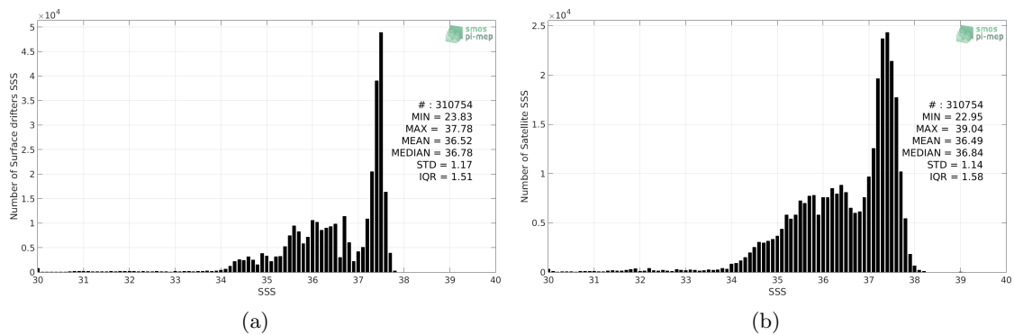
Figure 2: Histograms of SSS from Surface drifters (a) and SMOS L3 v317 - 10 Days - 25 km (CATDS-CPDC) (b) considering all match-up pairs per bins of 0.1 over the Tropical Atlantic Ocean Pi-MEP region and for the full satellite product period.
