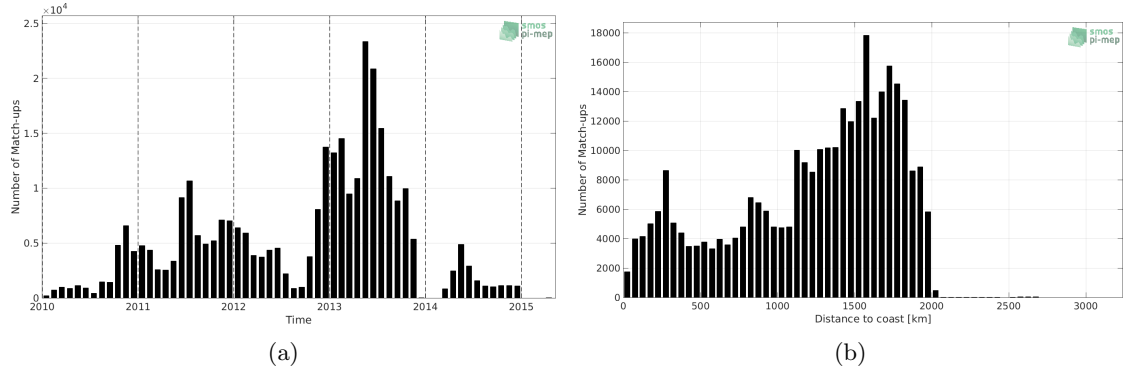
Figure 1: Number of match-ups between Surface drifters and SMOS L3 v317 - 10 Days - 25 km (CATDS-CPDC) SSS as a function of time (a) and as function of the distance to coast (b) over the Tropical Atlantic Ocean Pi-MEP region and for the full satellite product period.
