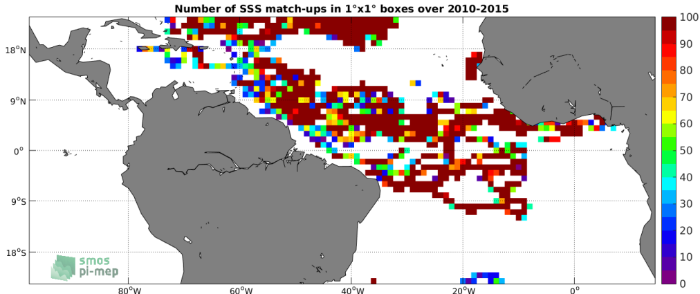
Figure 3: Number of SSS match-ups between Surface drifters SSS and the SMOS L3 v317 - 10 Days - 25 km (CATDS-CPDC) SSS product for the Tropical Atlantic Ocean Pi-MEP region over 1^\circ \times 1^\circ boxes and for the full satellite product period.
