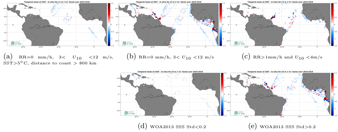
Figure 12: Temporal mean gridded over spatial boxes of size 1^\circ \times 1^\circ of \Delta SSS (SMOS-L3-CATDS-CPDC-V3-MONTHLY-25KM - TSG-LEGOS-DM) for 5 different subdatasets corresponding to: RR=0 mm/h, 3 < U_{10} < 12 m/s, SST > 5^\circ C , distance to coast > 800 km (a), RR=0 mm/h, 3 < U_{10} < 12 m/s (b), RR > 1 mm/h and U_{10} < 4 m/s (c), WOA2013 SSS Std < 0.2 (d), WOA2013 SSS Std > 0.2 (e).
