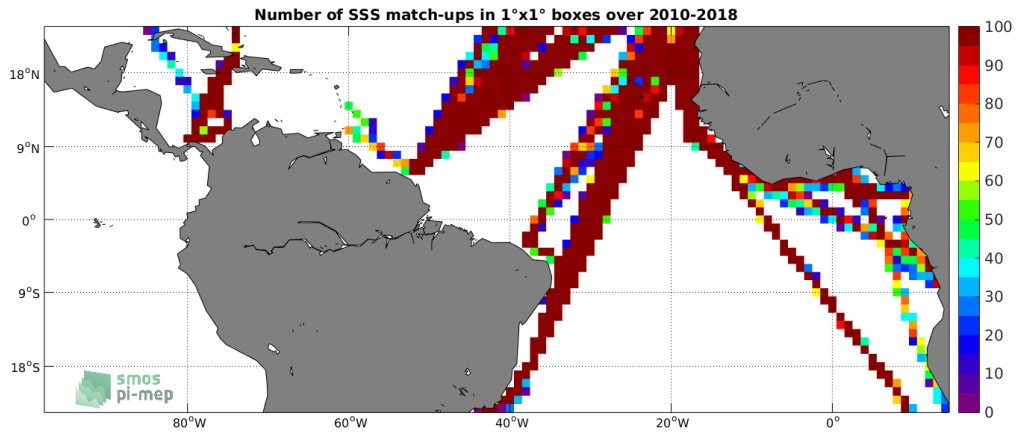
Figure 4: Number of SSS match-ups between TSG-LEGOS-DM SSS and the SMOS-L3-CATDS-CPDC-V3-MONTHLY-25KM SSS product for the Tropical Atlantic Ocean Pi-MEP region over 1^\circ \times 1^\circ boxes and for the full satellite product period.
