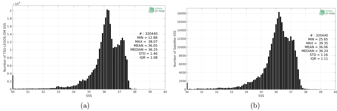
Figure 2: Histograms of SSS from TSG-LEGOS-DM (a) and SMOS-L3-CATDS-CPDC-V3-MONTHLY-25KM (b) considering all match-up pairs per bins of 0.1 over the Tropical Atlantic Ocean Pi-MEP region and for the full satellite product period.
