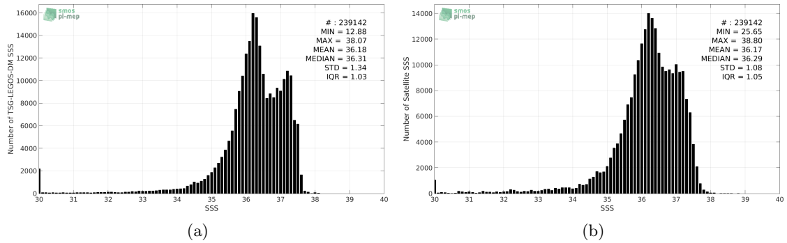
Figure 2: Histograms of SSS from TSG-LEGOS-DM (a) and SMOS-L3-CATDS-CPDC-V3-MONTHLY-25KM (b) considering all match-up pairs per bins of 0.1 over the Tropical Atlantic Ocean Pi-MEP region and for the full satellite product period.
