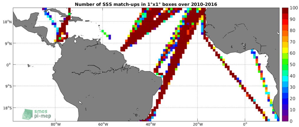
Figure 4: Number of SSS match-ups between TSG-LEGOS-DM SSS and the SMOS-L3-CATDS-CPDC-V3-MONTHLY-25KM SSS product for the Tropical Atlantic Ocean Pi-MEP region over 1°x1° boxes and for the full satellite product period.
