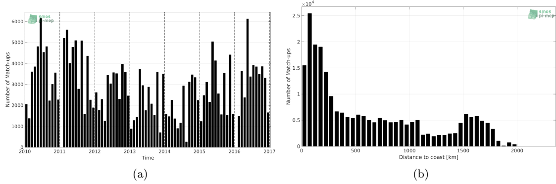
Figure 1: Number of match-ups between TSG-LEGOS-DM and SMOS-L3-CATDS-CPDC-V3-MONTHLY-25KM SSS as a function of time (a) and as function of the distance to coast (b) over the Tropical Atlantic Ocean Pi-MEP region and for the full satellite product period.
