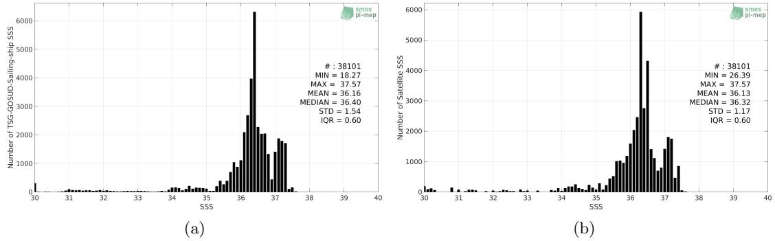
Figure 2: Histograms of SSS from TSG-GOSUD-Sailing-ship (a) and SMOS-L3-CATDS-CPDC-V3-MONTHLY-25KM (b) considering all match-up pairs per bins of 0.1 over the Tropical Atlantic Ocean Pi-MEP region and for the full satellite product period.
