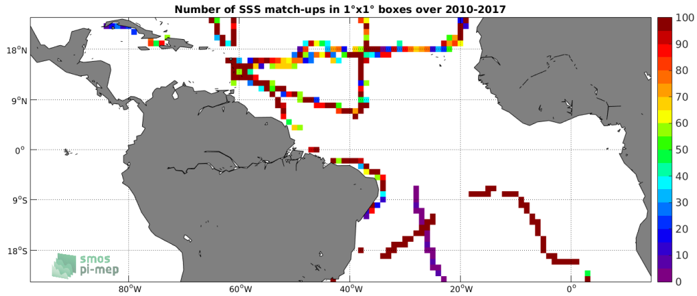
Figure 4: Number of SSS match-ups between TSG-GOSUD-Sailing-ship SSS and the SMOS-L3-CATDS-CPDC-V3-MONTHLY-25KM SSS product for the Tropical Atlantic Ocean Pi-MEP region over 1°x1° boxes and for the full satellite product period.
