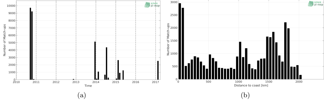
Figure 1: Number of match-ups between TSG-GOSUD-Sailing-ship and SMOS-L3-CATDS-CPDC-V3-MONTHLY-25KM SSS as a function of time (a) and as function of the distance to coast (b) over the Tropical Atlantic Ocean Pi-MEP region and for the full satellite product period.
