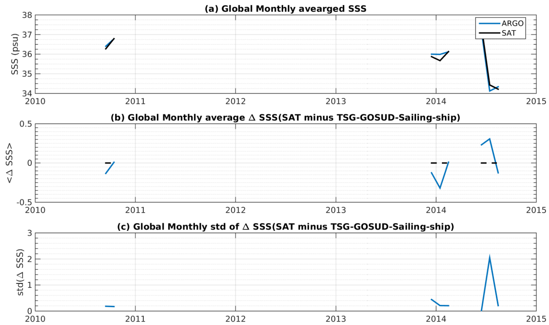
Figure 7: Time series of the monthly averaged mean SSS (top), mean \Delta \text{SSS} (Satellite - TSG-GOSUD-Sailing-ship) and STD of \Delta \text{SSS} (Satellite - TSG-GOSUD-Sailing-ship) over the Tropical Atlantic Ocean Pi-MEP region considering all match-ups collected by the Pi-MEP platform.
