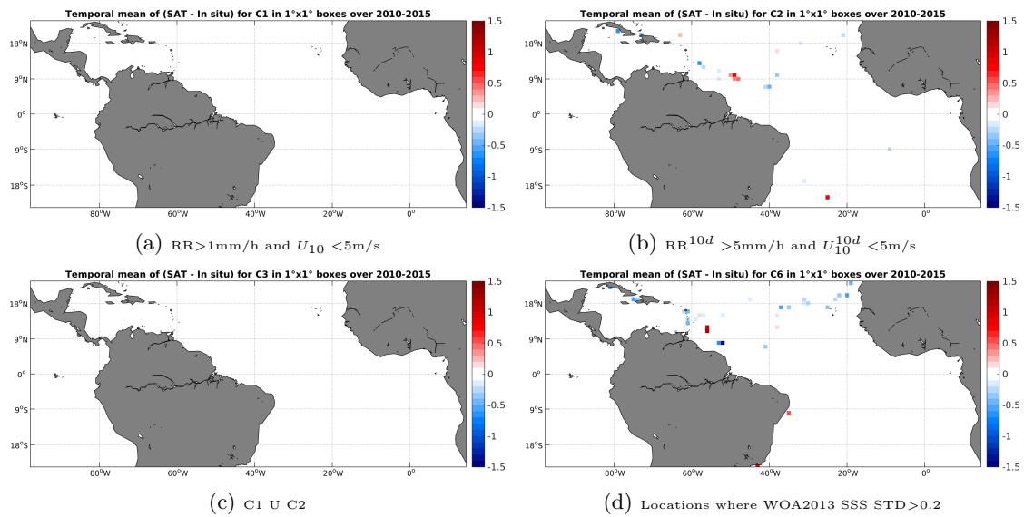
Figure 12: Temporal mean gridded over spatial boxes of size 1^\circ \times 1^\circ of \Delta SSS (SMOS-L3-CATDS-CPDC-V3-MONTHLY-25KM - TSG-GOSUD-Sailing-ship) for 4 different subdatasets corresponding to: RR > 1\text{mm/h} and U_{10} < 5\text{m/s} (a), RR^{10d} > 5\text{mm/h} and U_{10}^{10d} < 5\text{m/s} (b), C1 U C2 (c), Locations where WOA2013 SSS STD > 0.2 (d).
