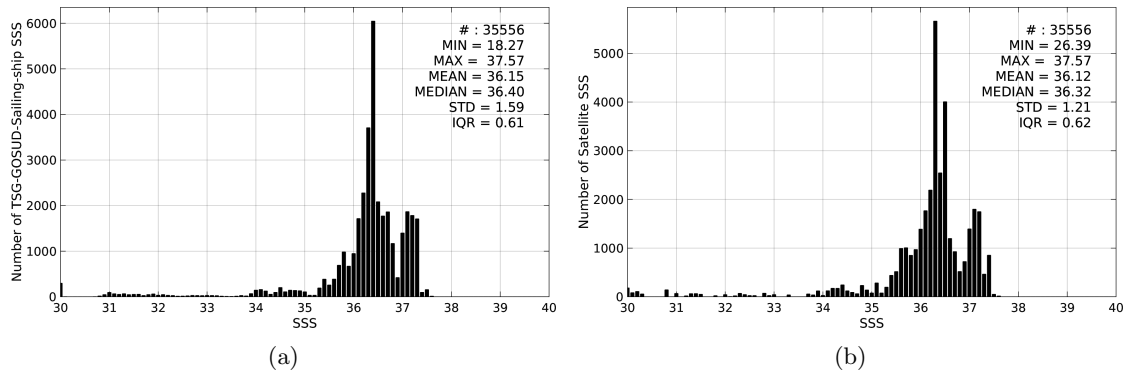
Figure 2: Histograms of SSS from TSG-GOSUD-Sailing-ship (a) and SMOS-L3-CATDS-CPDC-V3-MONTHLY-25KM (b) considering all match-up pairs per bins of 0.1 over the Tropical Atlantic Ocean Pi-MEP region and for the full satellite product period.
