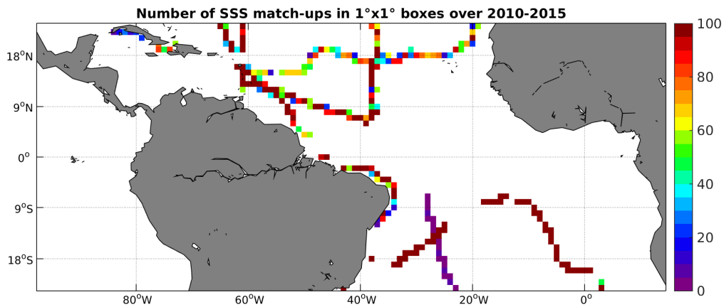
Figure 4: Number of SSS match-ups between TSG-GOSUD-Sailing-ship SSS and the SMOS-L3-CATDS-CPDC-V3-MONTHLY-25KM SSS product for the Tropical Atlantic Ocean Pi-MEP region over 1^\circ \times 1^\circ boxes and for the full satellite product period.
