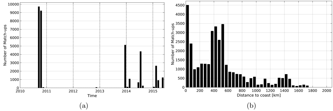
Figure 1: Number of match-ups between TSG-GOSUD-Sailing-ship and SMOS-L3-CATDS-CPDC-V3-MONTHLY-25KM SSS as a function of time (a) and as function of the distance to coast (b) over the Tropical Atlantic Ocean Pi-MEP region and for the full satellite product period.
