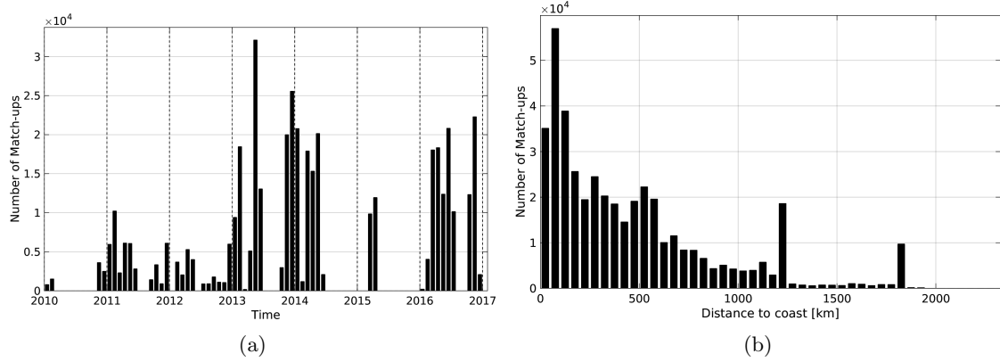
Figure 1: Number of match-ups between TSG-GOSUD-Research-vessel and SMOS-L3-CATDS-CPDC-V3-MONTHLY-25KM SSS as a function of time (a) and as function of the distance to coast (b) over the Tropical Atlantic Ocean Pi-MEP region and for the full satellite product period.
