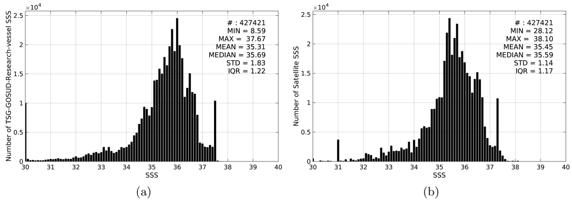
Figure 2: Histograms of SSS from TSG-GOSUD-Research-vessel (a) and SMOS-L3-CATDS-CPDC-V3-MONTHLY-25KM (b) considering all match-up pairs per bins of 0.1 over the Tropical Atlantic Ocean Pi-MEP region and for the full satellite product period.
