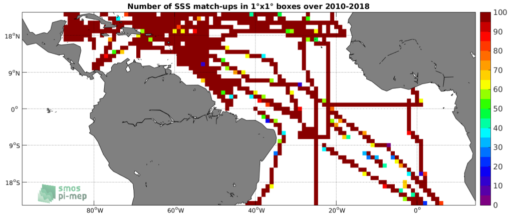
Figure 4: Number of SSS match-ups between TSG-SAMOS SSS and the SMOS-L3-CATDS-CPDC-V3-10DAYS-25KM SSS product for the Tropical Atlantic Ocean Pi-MEP region over 1°x1° boxes and for the full satellite product period.
