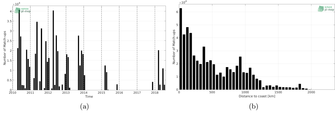
Figure 1: Number of match-ups between TSG-SAMOS and SMOS-L3-CATDS-CPDC-V3-10DAYS-25KM SSS as a function of time (a) and as function of the distance to coast (b) over the Tropical Atlantic Ocean Pi-MEP region and for the full satellite product period.
