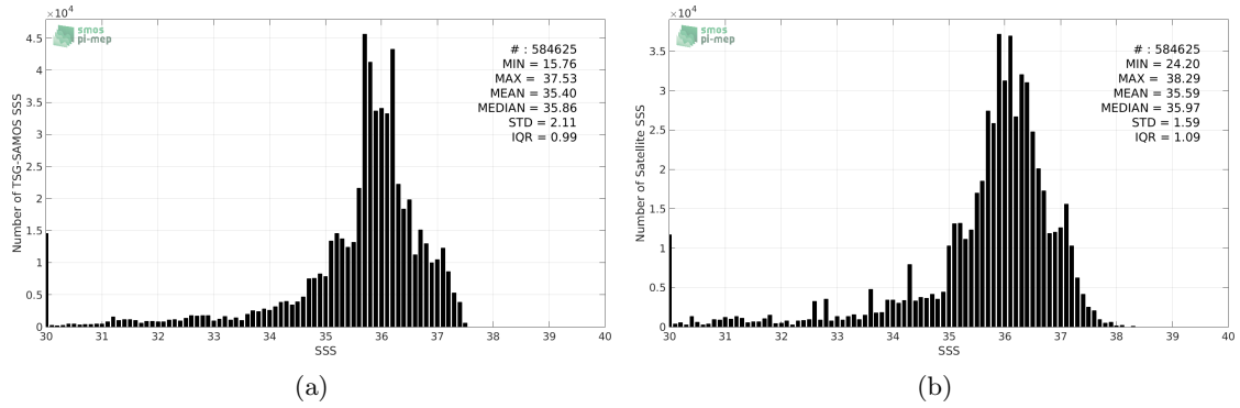
Figure 2: Histograms of SSS from TSG-SAMOS (a) and SMOS-L3-CATDS-CPDC-V3-10DAYS-25KM (b) considering all match-up pairs per bins of 0.1 over the Tropical Atlantic Ocean Pi-MEP region and for the full satellite product period.
