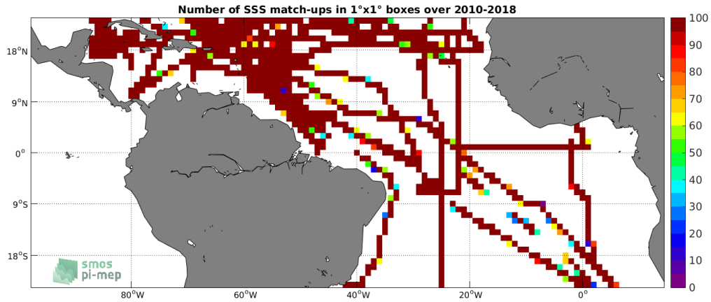
Figure 4: Number of SSS match-ups between TSG-SAMOS SSS and the SMOS-L3-CATDS-CPDC-V3-10DAYS-25KM SSS product for the Tropical Atlantic Ocean Pi-MEP region over 1^\circ \times 1^\circ boxes and for the full satellite product period.
