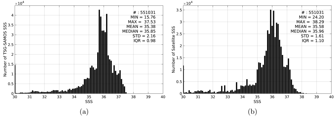
Figure 2: Histograms of SSS from TSG-SAMOS (a) and SMOS-L3-CATDS-CPDC-V3-10DAYS-25KM (b) considering all match-up pairs per bins of 0.1 over the Tropical Atlantic Ocean Pi-MEP region and for the full satellite product period.
