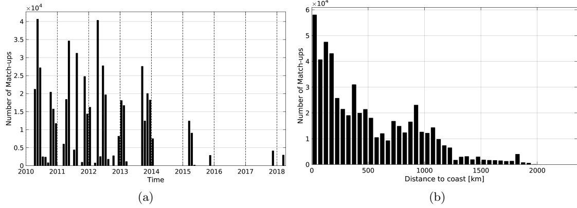
Figure 1: Number of match-ups between TSG-SAMOS and SMOS-L3-CATDS-CPDC-V3-10DAYS-25KM SSS as a function of time (a) and as function of the distance to coast (b) over the Tropical Atlantic Ocean Pi-MEP region and for the full satellite product period.
