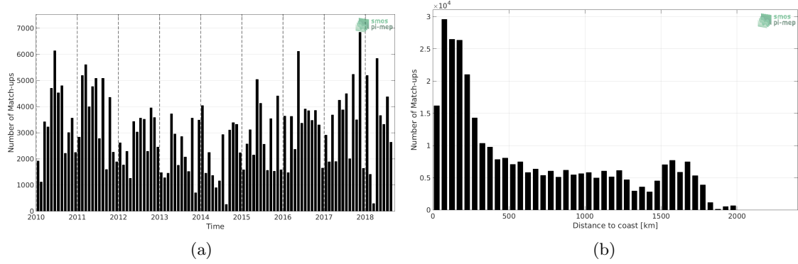
Figure 1: Number of match-ups between TSG-LEGOS-DM and SMOS-L3-CATDS-CPDC-V3-10DAYS-25KM SSS as a function of time (a) and as function of the distance to coast (b) over the Tropical Atlantic Ocean Pi-MEP region and for the full satellite product period.
