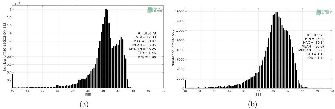
Figure 2: Histograms of SSS from TSG-LEGOS-DM (a) and SMOS-L3-CATDS-CPDC-V3-10DAYS-25KM (b) considering all match-up pairs per bins of 0.1 over the Tropical Atlantic Ocean Pi-MEP region and for the full satellite product period.
