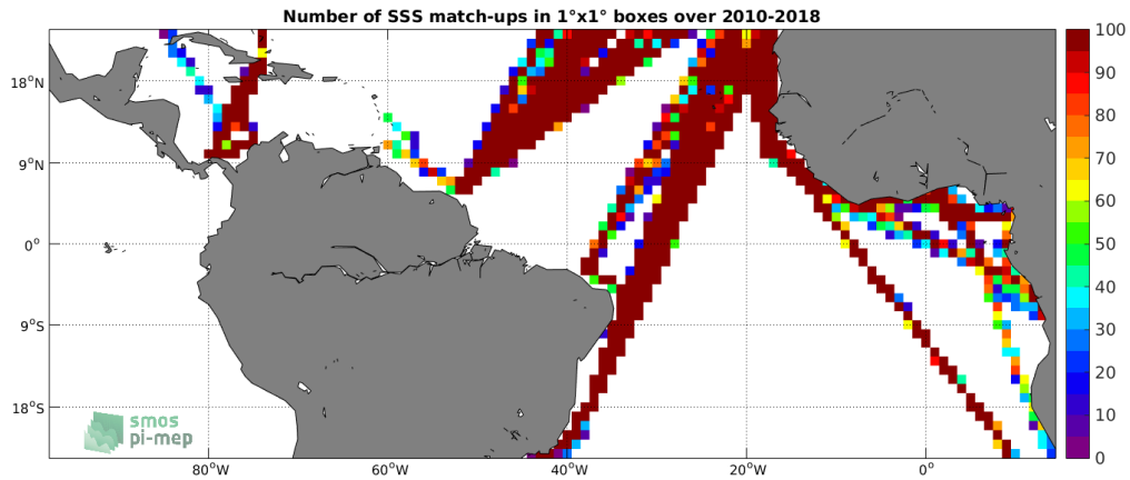
Figure 4: Number of SSS match-ups between TSG-LEGOS-DM SSS and the SMOS-L3-CATDS-CPDC-V3-10DAYS-25KM SSS product for the Tropical Atlantic Ocean Pi-MEP region over 1^\circ \times 1^\circ boxes and for the full satellite product period.
