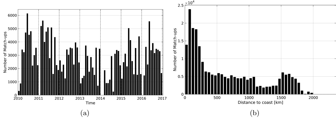
Figure 1: Number of match-ups between TSG-LEGOS-DM and SMOS-L3-CATDS-CPDC-V3-10DAYS-25KM SSS as a function of time (a) and as function of the distance to coast (b) over the Tropical Atlantic Ocean Pi-MEP region and for the full satellite product period.
