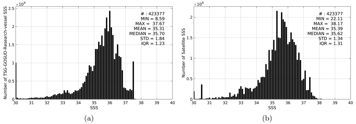
Figure 2: Histograms of SSS from TSG-GOSUD-Research-vessel (a) and SMOS-L3-CATDS-CPDC-V3-10DAYS-25KM (b) considering all match-up pairs per bins of 0.1 over the Tropical Atlantic Ocean Pi-MEP region and for the full satellite product period.
