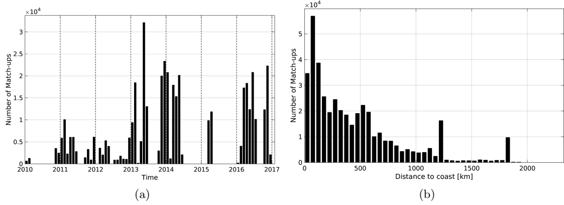
Figure 1: Number of match-ups between TSG-GOSUD-Research-vessel and SMOS-L3-CATDS-CPDC-V3-10DAYS-25KM SSS as a function of time (a) and as function of the distance to coast (b) over the Tropical Atlantic Ocean Pi-MEP region and for the full satellite product period.
