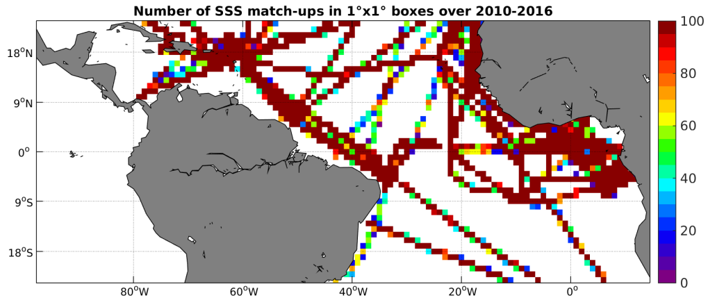
Figure 4: Number of SSS match-ups between TSG-GOSUD-Research-vessel SSS and the SMOS-L3-CATDS-CPDC-V3-10DAYS-25KM SSS product for the Tropical Atlantic Ocean Pi-MEP region over 1°x1° boxes and for the full satellite product period.
