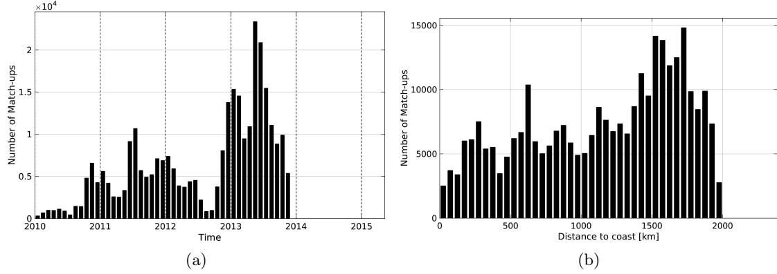
Figure 1: Number of match-ups between Surface drifters and SMOS-L3-CATDS-CPDC-V3-10DAYS-25KM SSS as a function of time (a) and as function of the distance to coast (b) over the Tropical Atlantic Ocean Pi-MEP region and for the full satellite product period.
