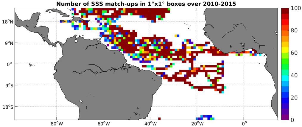
Figure 3: Number of SSS match-ups between Surface drifters SSS and the SMOS-L3-CATDS-CPDC-V3-10DAYS-25KM SSS product for the Tropical Atlantic Ocean Pi-MEP region over 1^\circ \times 1^\circ boxes and for the full satellite product period.
