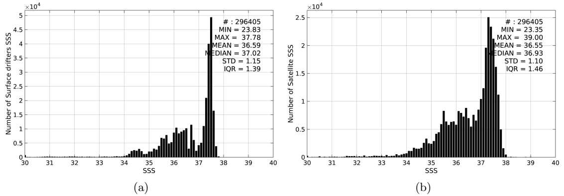
Figure 2: Histograms of SSS from Surface drifters (a) and SMOS-L3-CATDS-CPDC-V3-10DAYS-25KM (b) considering all match-up pairs per bins of 0.1 over the Tropical Atlantic Ocean Pi-MEP region and for the full satellite product period.
