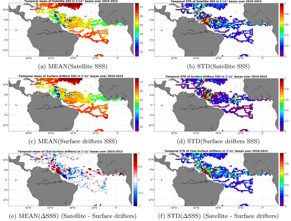
Figure 5: Temporal mean (left) and STD (right) of SSS from SMOS-L3-CATDS-CPDC-V3-10DAYS-25KM (top), Surface drifters (middle), and of \Delta\text{SSS} (Satellite - Surface drifters). Only match-up pairs are used to generate these maps.
