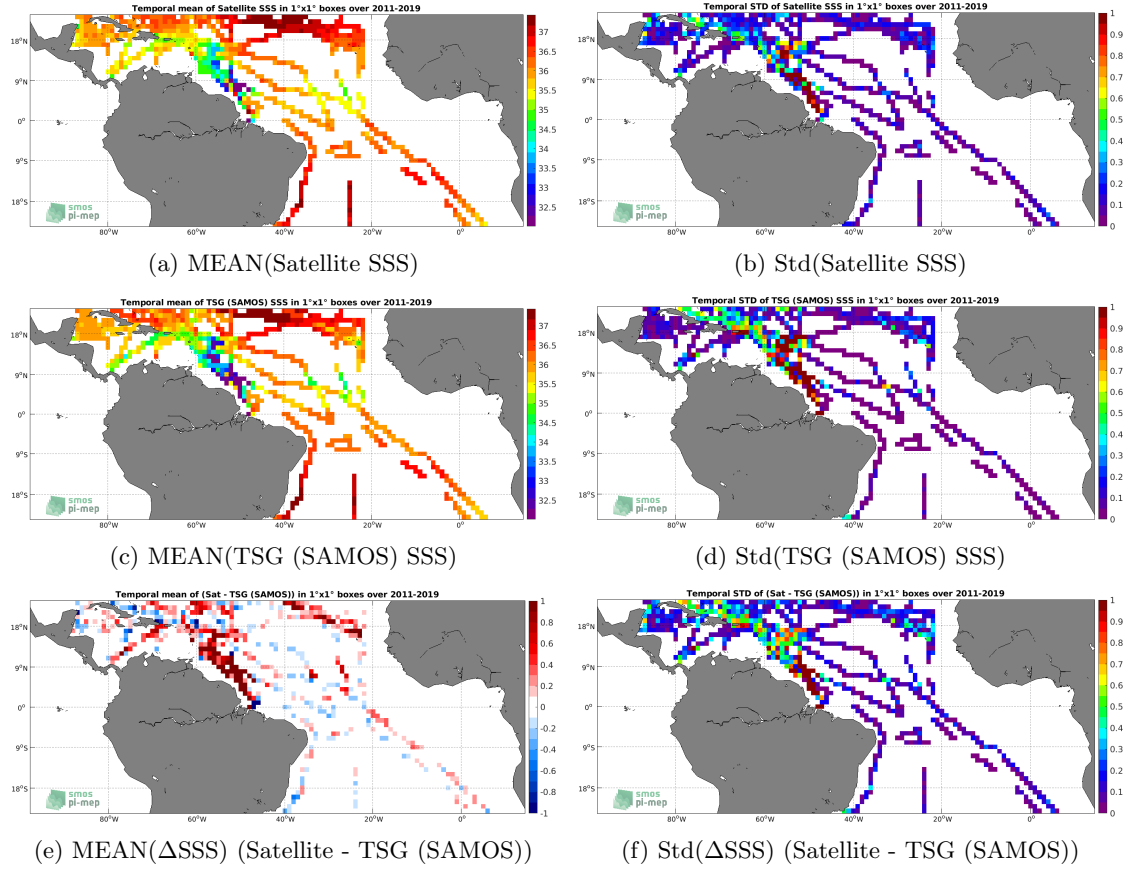
Figure 6: Temporal mean (left) and Std (right) of SSS from SMOS SSS L3 v2 - 9-Days (BEC) (top), TSG (SAMOS) (middle), and of \Delta SSS (Satellite - TSG (SAMOS)). Only match-up pairs are used to generate these maps.
