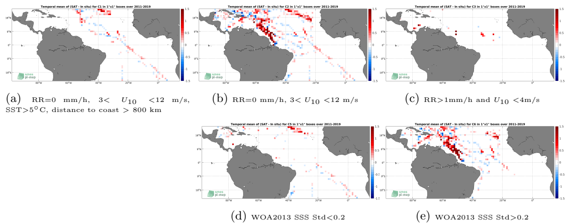
Figure 12: Temporal mean gridded over spatial boxes of size 1^\circ \times 1^\circ of \Delta SSS (SMOS SSS L3 v2 - 9-Days (BEC) - TSG (SAMOS)) for 5 different subdatasets corresponding to:RR=0 mm/h, 3 < U_{10} < 12 m/s, SST >5^\circ\text{C} , distance to coast > 800 km (a), RR=0 mm/h, 3 < U_{10} < 12 m/s (b), RR >1 mm/h and U_{10} < 4 m/s (c), WOA2013 SSS Std <0.2 (d), WOA2013 SSS Std >0.2 (e).
