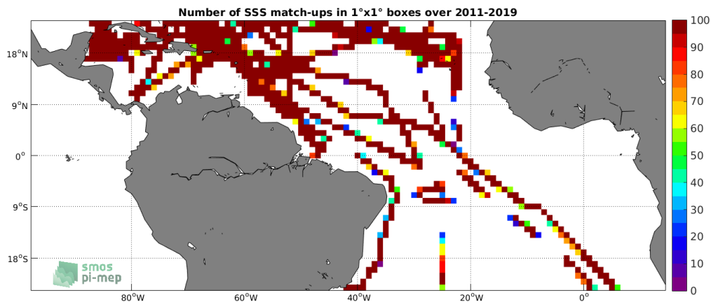
Figure 4: Number of SSS match-ups between TSG (SAMOS) SSS and the SMOS L3 v2 - 9-Days (BEC) SSS product for the Tropical Atlantic Ocean Pi-MEP region over 1^\circ \times 1^\circ boxes and for the full satellite product period.
