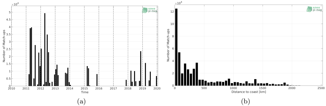
Figure 1: Number of match-ups between TSG (SAMOS) and SMOS L3 v2 - 9-Days (BEC) SSS as a function of time (a) and as function of the distance to coast (b) over the Tropical Atlantic Ocean Pi-MEP region and for the full satellite product period.
