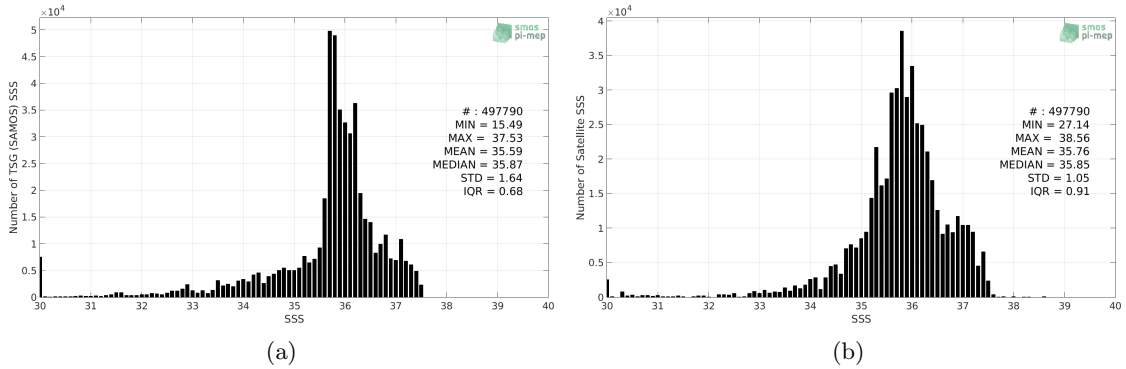
Figure 2: Histograms of SSS from TSG (SAMOS) (a) and SMOS L3 v2 - 9-Days (BEC) (b) considering all match-up pairs per bins of 0.1 over the Tropical Atlantic Ocean Pi-MEP region and for the full satellite product period.
