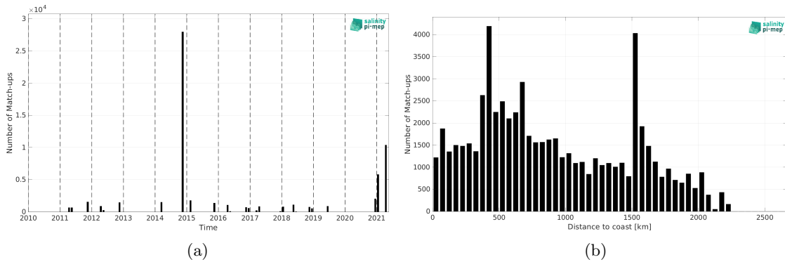
Figure 2: Number of match-ups between TSG (Polarstern) and SMOS SSS L3 v2 - 9-Days (BEC) SSS as a function of time (a) and as function of the distance to coast (b) over the Tropical Atlantic Ocean Pi-MEP region and for the full satellite product period.
