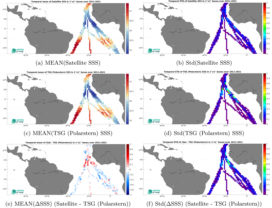
Figure 7: Temporal mean (left) and Std (right) of SSS from SMOS SSS L3 v2 - 9-Days (BEC) (top), TSG (Polarstern) (middle), and of \Delta\text{SSS} (Satellite - TSG (Polarstern)). Only match-up pairs are used to generate these maps.
