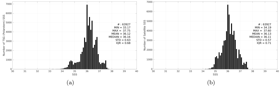
Figure 3: Histograms of SSS from TSG (Polarstern) (a) and SMOS SSS L3 v2 - 9-Days (BEC) (b) considering all match-up pairs per bins of 0.1 over the Tropical Atlantic Ocean Pi-MEP region and for the full satellite product period.
