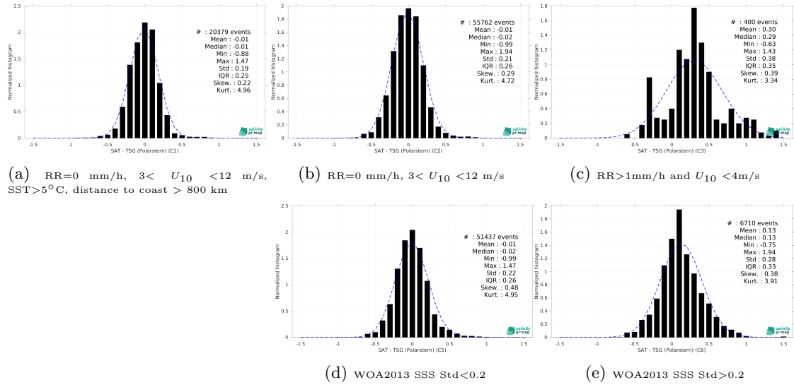
Figure 15: Normalized histogram of \Delta SSS (SMOS SSS L3 v2 - 9-Days (BEC) - TSG (Polarstern)) for 5 different subdatasets corresponding to: RR=0 mm/h, 3 < U_{10} < 12 m/s, SST>5°C, distance to coast > 800 km (a), RR=0 mm/h, 3 < U_{10} < 12 m/s (b), RR>1mm/h and U_{10} < 4 m/s (c), WOA2013 SSS Std<0.2 (d), WOA2013 SSS Std>0.2 (e).
