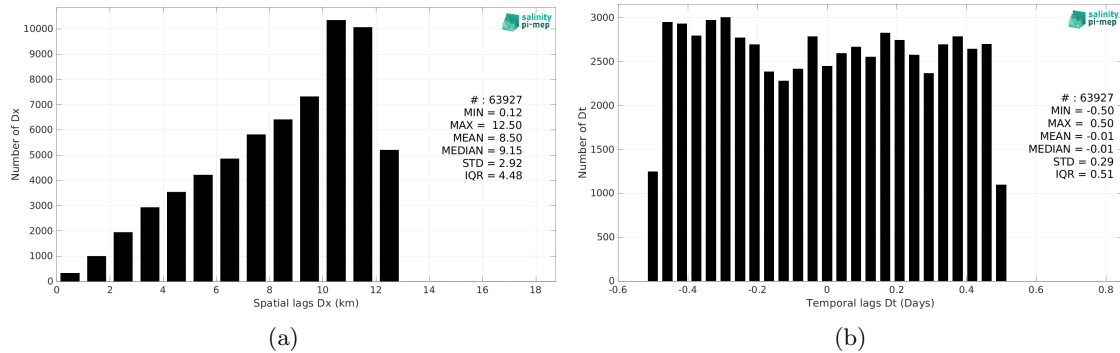
Figure 6: Histograms of the spatial (a) and temporal (b) lags between the location/time of the TSG (Polarstern) measurement and the date of the corresponding SMOS SSS L3 v2 - 9-Days (BEC) SSS pixel.
