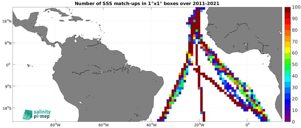
Figure 5: Number of SSS match-ups between TSG (Polarstern) SSS and the SMOS SSS L3 v2 - 9-Days (BEC) SSS product for the Tropical Atlantic Ocean Pi-MEP region over 1^\circ \times 1^\circ boxes and for the full satellite product period.
