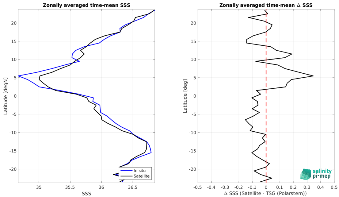
Figure 9: Left panel: Zonal mean SSS from SMOS SSS L3 v2 - 9-Days (BEC) satellite product (black) and from TSG (Polarstern) (blue). Right panel: Zonal mean of \Delta SSS (Satellite - TSG (Polarstern)) for all the collected Pi-MEP match-up pairs estimated over the full satellite product period.
