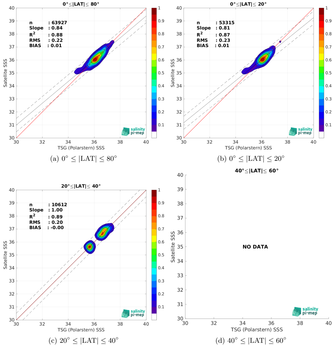
Figure 10: Contour maps of the concentration of SMOS SSS L3 v2 - 9-Days (BEC) SSS (y-axis) versus TSG (Polarstern) SSS (x-axis) at match-up pairs for different latitude bands. For each plot, the red line shows x=y . The black thin and dashed lines indicate a linear fit through the data cloud and the \pm 95\% confidence levels, respectively. The number match-up pairs n , the slope and R^2 coefficient of the linear fit, the root mean square (RMS) and the mean bias between satellite and in situ data are indicated for each latitude band in each plots.
