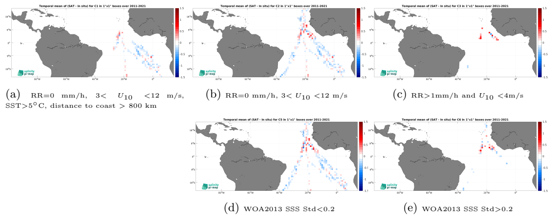
Figure 14: Temporal mean gridded over spatial boxes of size 1^\circ \times 1^\circ of \Delta SSS (SMOS SSS L3 v2 - 9-Days (BEC) - TSG (Polarstern)) for 5 different subdatasets corresponding to:RR=0 mm/h, 3 < U_{10} < 12 m/s, SST >5^\circ\text{C} , distance to coast > 800 km (a), RR=0 mm/h, 3 < U_{10} < 12 m/s (b), RR >1 mm/h and U_{10} < 4 m/s (c), WOA2013 SSS Std <0.2 (d), WOA2013 SSS Std >0.2 (e).
