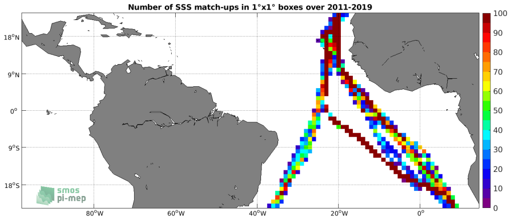
Figure 4: Number of SSS match-ups between TSG (Polarstern) SSS and the SMOS SSS L3 v2 - 9-Days (BEC) SSS product for the Tropical Atlantic Ocean Pi-MEP region over 1°x1° boxes and for the full satellite product period.
