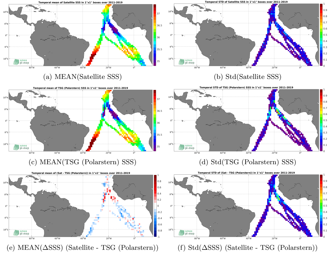
Figure 6: Temporal mean (left) and Std (right) of SSS from SMOS SSS L3 v2 - 9-Days (BEC) (top), TSG (Polarstern) (middle), and of \Delta SSS (Satellite - TSG (Polarstern)). Only match-up pairs are used to generate these maps.
