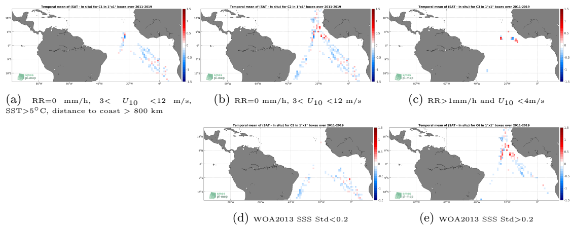
Figure 12: Temporal mean gridded over spatial boxes of size 1^\circ \times 1^\circ of \Delta SSS (SMOS SSS L3 v2 - 9-Days (BEC) - TSG (Polarstern)) for 5 different subdatasets corresponding to: RR=0 mm/h, 3 < U_{10} < 12 m/s, SST > 5^\circ\text{C} , distance to coast > 800 km (a), RR=0 mm/h, 3 < U_{10} < 12 m/s (b), RR > 1 mm/h and U_{10} < 4 m/s (c), WOA2013 SSS Std < 0.2 (d), WOA2013 SSS Std > 0.2 (e).
