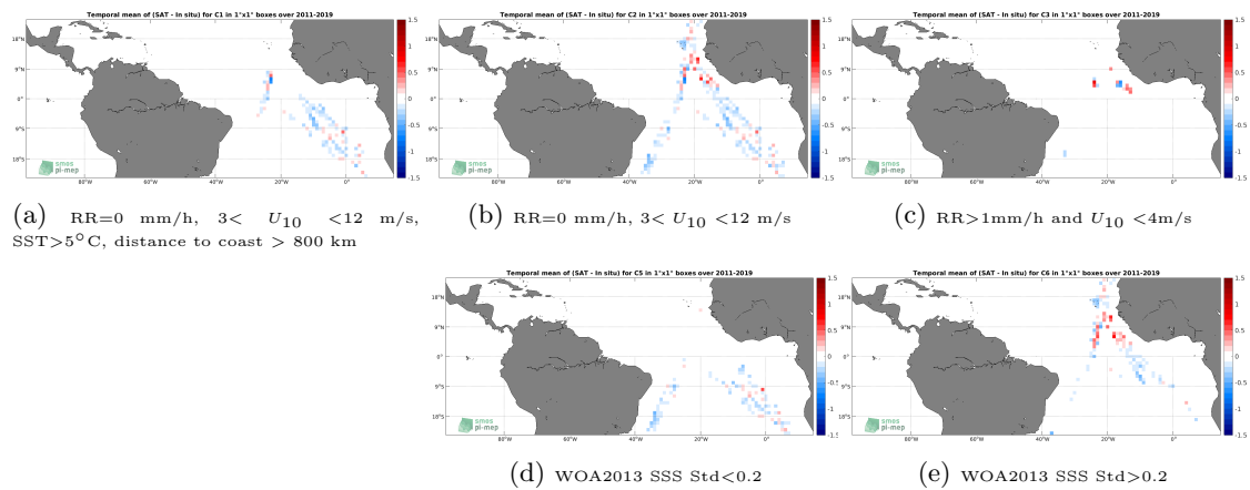
Figure 12: Temporal mean gridded over spatial boxes of size 1^\circ \times 1^\circ of \Delta\text{SSS} (SMOS SSS L3 v2 - 9-Days (BEC) - TSG (Polarstern)) for 5 different subdatasets corresponding to:RR=0 mm/h, 3 < U_{10} < 12 m/s, SST >5^\circ\text{C} , distance to coast > 800 km (a), RR=0 mm/h, 3 < U_{10} < 12 m/s (b), RR >1 mm/h and U_{10} < 4 m/s (c), WOA2013 SSS Std <0.2 (d), WOA2013 SSS Std >0.2 (e).
