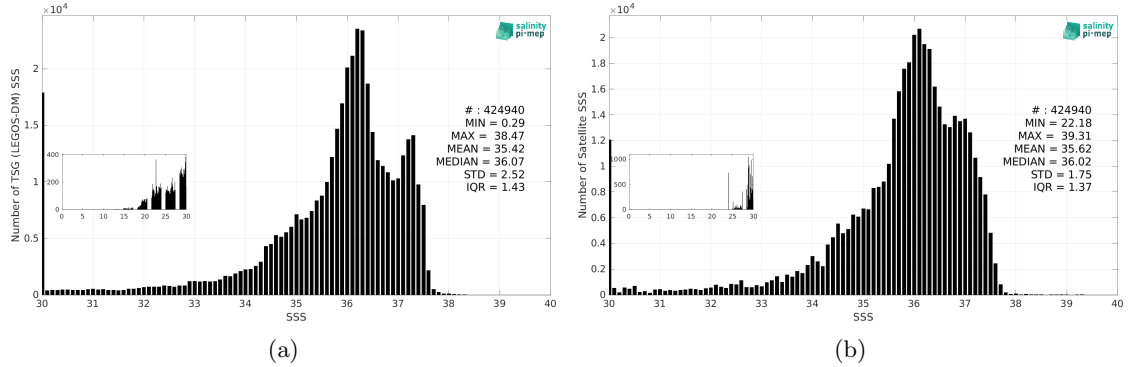
Figure 3: Histograms of SSS from TSG (LEGOS-DM) (a) and SMOS SSS L3 v2 - 9-Days (BEC) (b) considering all match-up pairs per bins of 0.1 over the Tropical Atlantic Ocean Pi-MEP region and for the full satellite product period.
