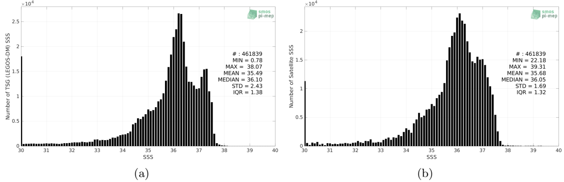
Figure 2: Histograms of SSS from TSG (LEGOS-DM) (a) and SMOS SSS L3 v2 - 9-Days (BEC) (b) considering all match-up pairs per bins of 0.1 over the Tropical Atlantic Ocean Pi-MEP region and for the full satellite product period.
