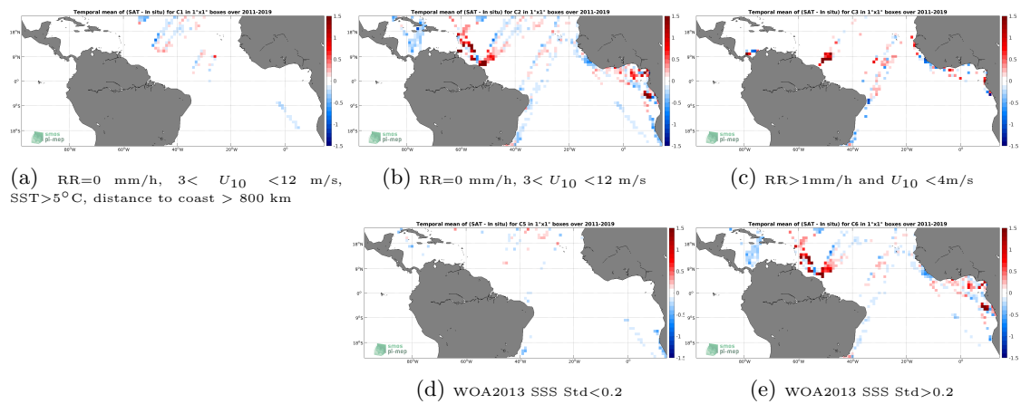
Figure 12: Temporal mean gridded over spatial boxes of size 1^\circ \times 1^\circ of \Delta\text{SSS} (SMOS SSS L3 v2 - 9-Days (BEC) - TSG (LEGOS-DM)) for 5 different subdatasets corresponding to:RR=0 mm/h, 3 < U_{10} < 12 m/s, SST >5^\circ\text{C} , distance to coast > 800 km (a), RR=0 mm/h, 3 < U_{10} < 12 m/s (b), RR >1 mm/h and U_{10} < 4 m/s (c), WOA2013 SSS Std <0.2 (d), WOA2013 SSS Std >0.2 (e).
